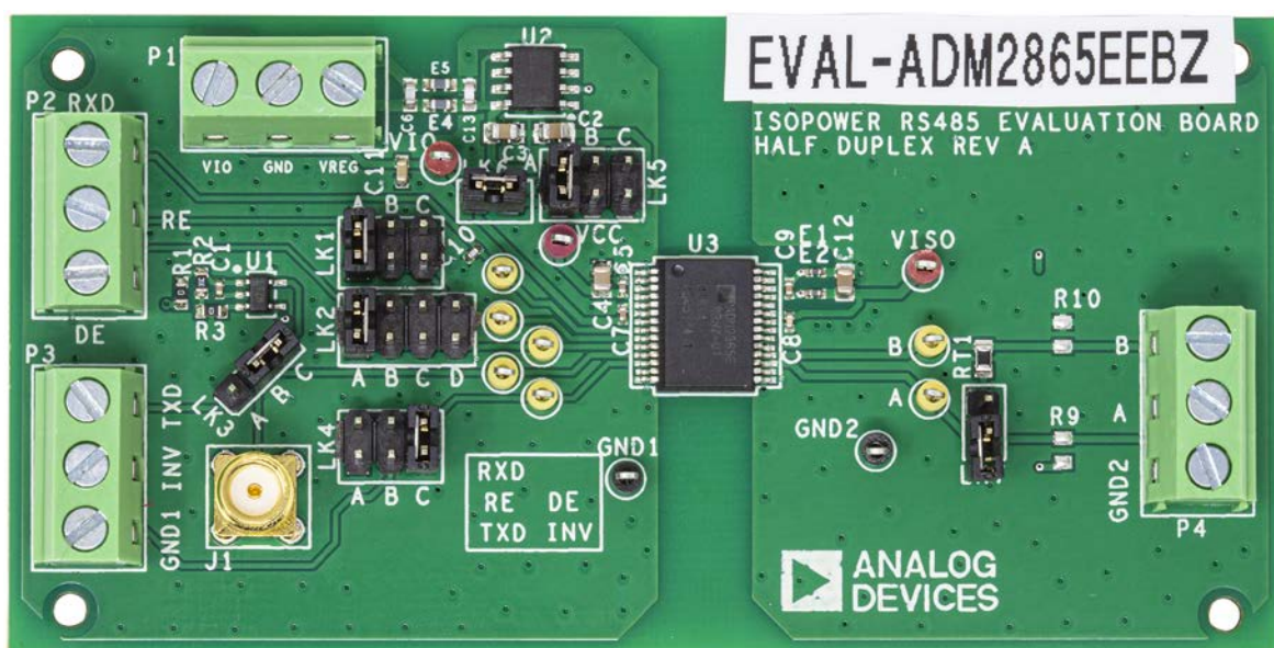
Figure 2. EVAL-ADM2865EEBZ
