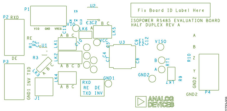
Figure 10. EVAL-ADM2565EEBZ/EVAL-ADM2865EEBZ, Silkscreen
