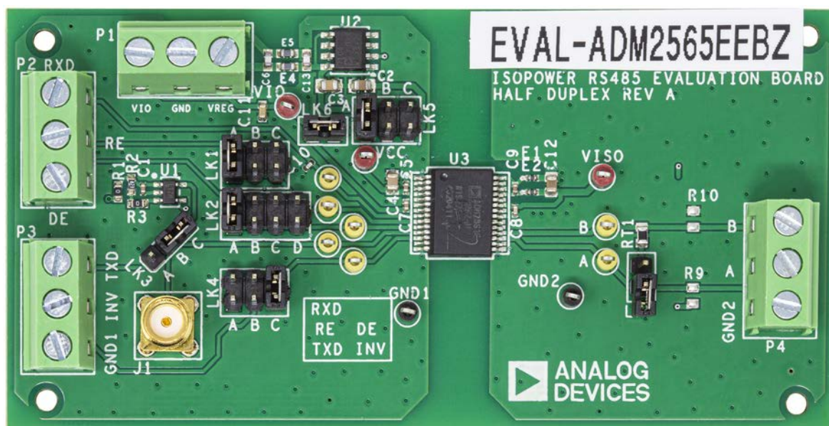
Figure 1. EVAL-ADM2565EEBZ
