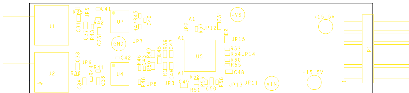
Figure 27. EVAL-ADAQ4001PMDZ and EVAL-ADAQ4003PMDZ Silkscreen, Top Layer
