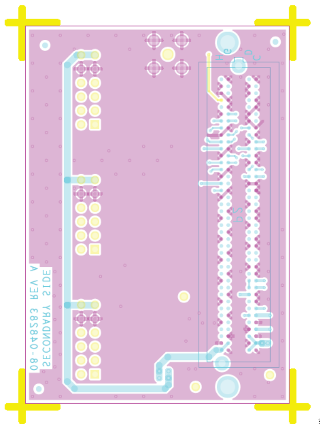
Figure 36. EVAL-PMD-IB1Z, Secondary
