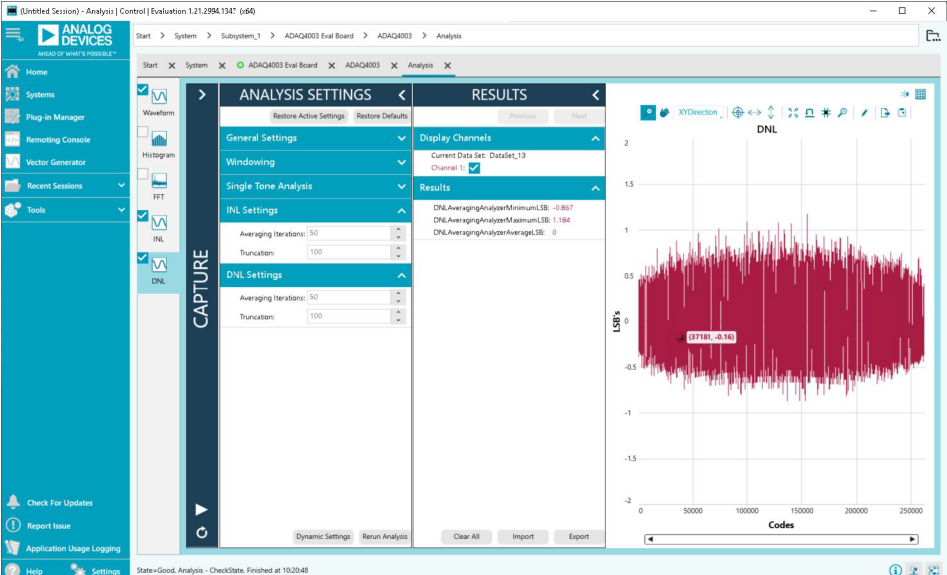
Figure 24. DNL Tab
