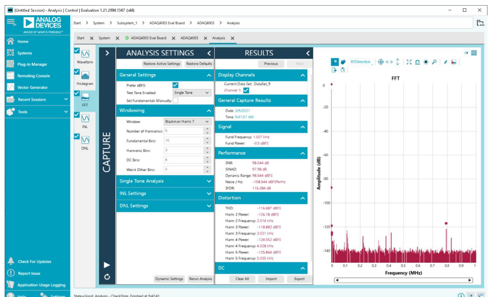
Figure 22. FFT Tab
