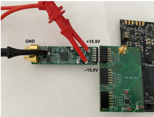
Figure 3. EVAL-ADAQ4001PMDZ and EVAL-ADAQ4003PMDZ External Supply (Optional) Connections
