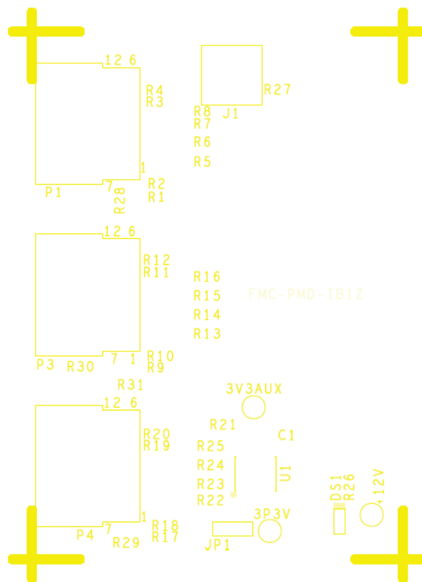
Figure 34. EVAL-PMD-IB1Z Silkscreen, Primary
