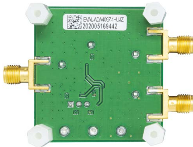
Figure 2. EVAL-ADA4097-1HUIZ, Secondary Side
