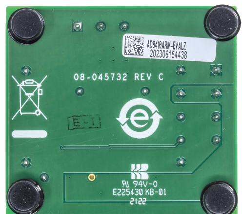
Figure 4. AD8410ARM-EVALZ Bottom View
