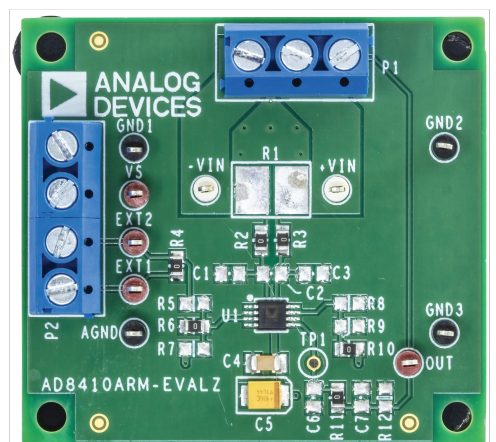
Figure 3. AD8410ARM-EVALZ Top View
