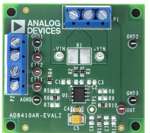
Figure 1. AD8410AR-EVALZ Top View
