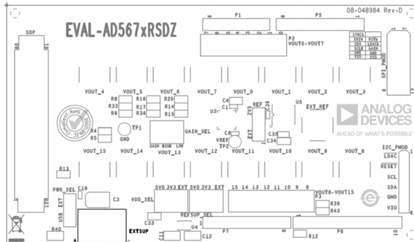
Figure 10. EVAL-AD5677RSDZ Top Side Component Placement
