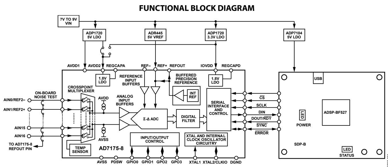
Figure 1. EVAL-AD7175-8SDZ Block Diagram
