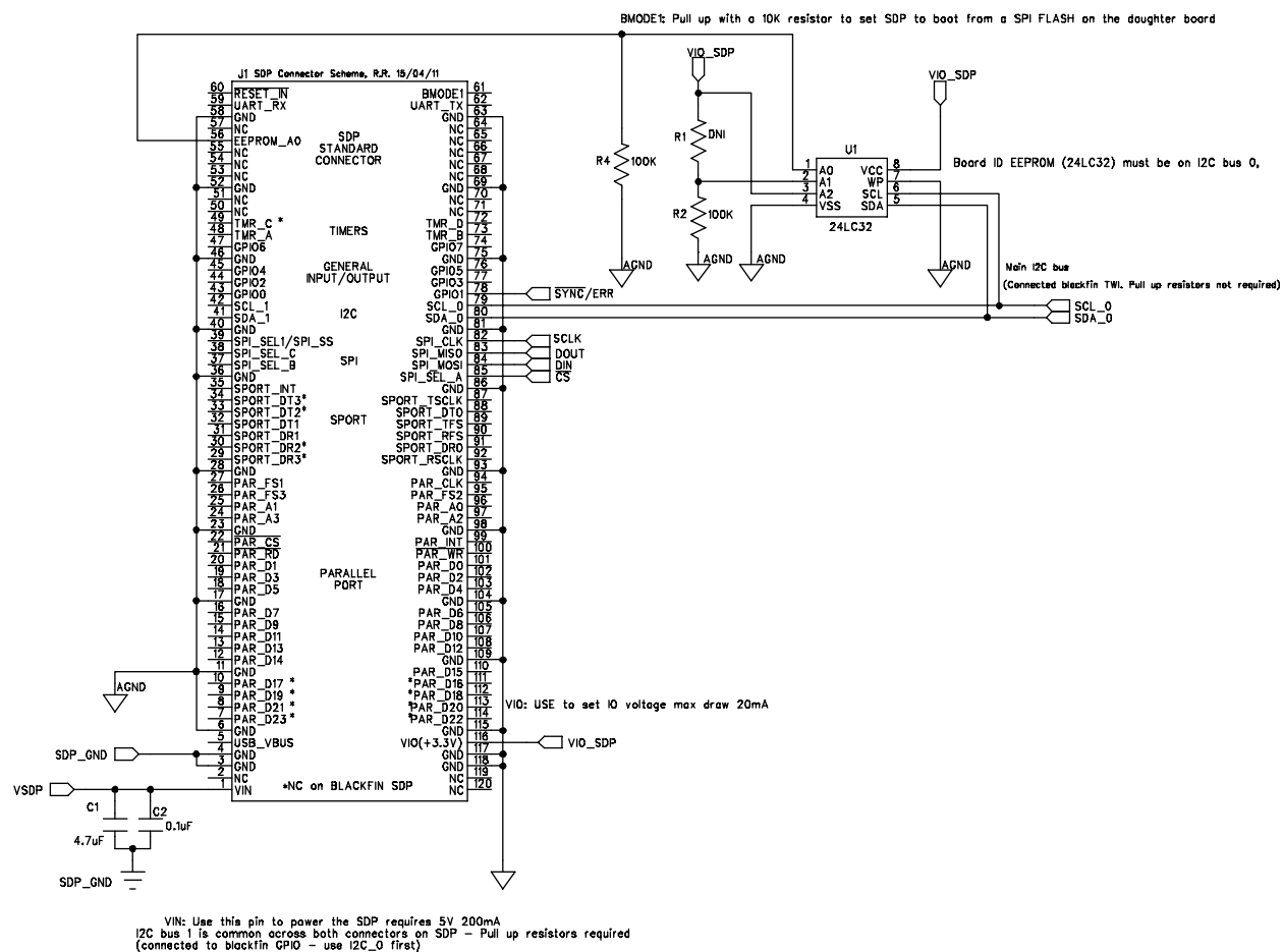
Figure 28. SDP-B Connector Schematic
