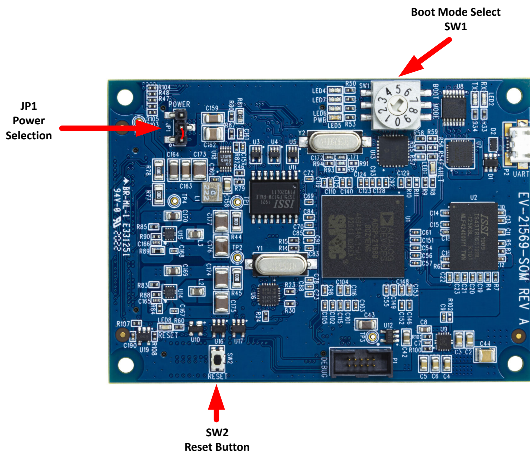
Figure 3-6: Switch/Jumper Locations
