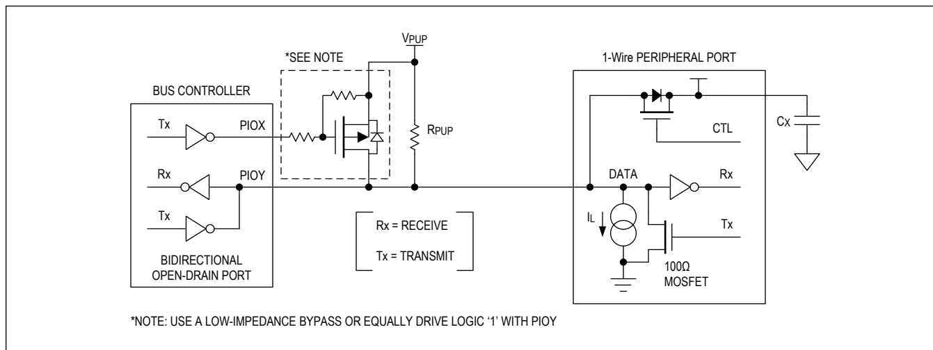
Figure 2. Hardware Configuration
