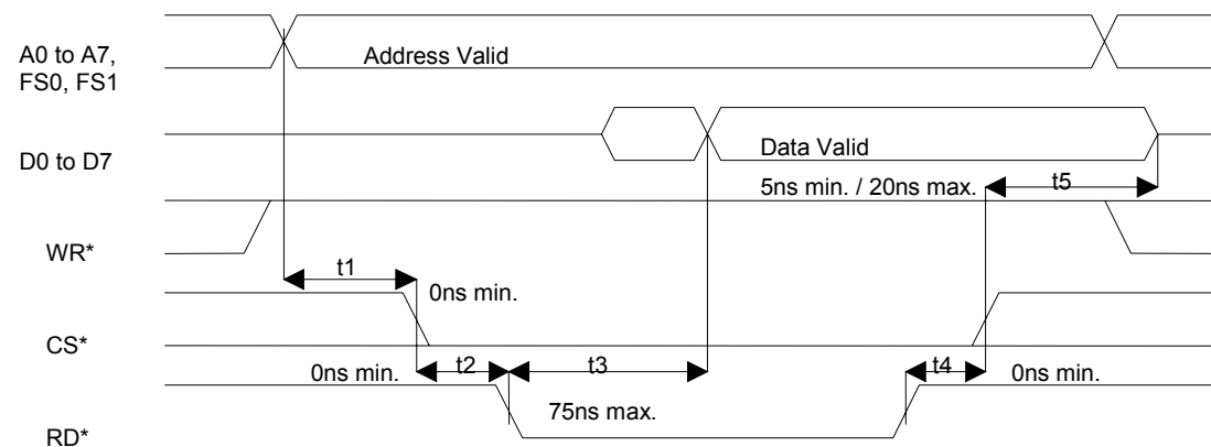
Figure 23-4. INTEL BUS READ AC TIMING (BTS = 0 / MUX = 0)
