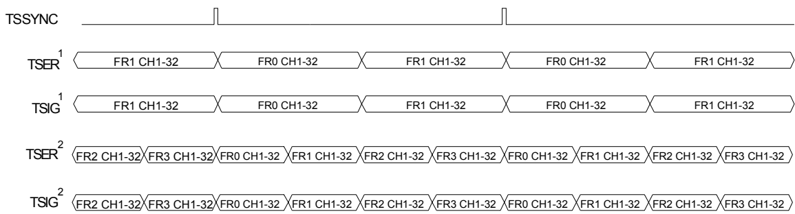
Figure 22-13. TRANSMIT SIDE INTERLEAVED BUS OPERATION FRAME MODE TIMING
