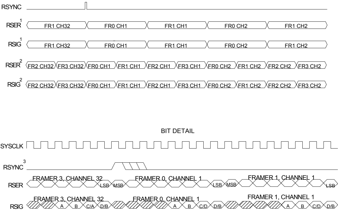
Figure 22-5. RECEIVE SIDE, INTERLEAVED BUS OPERATION BYTE MODE TIMING
