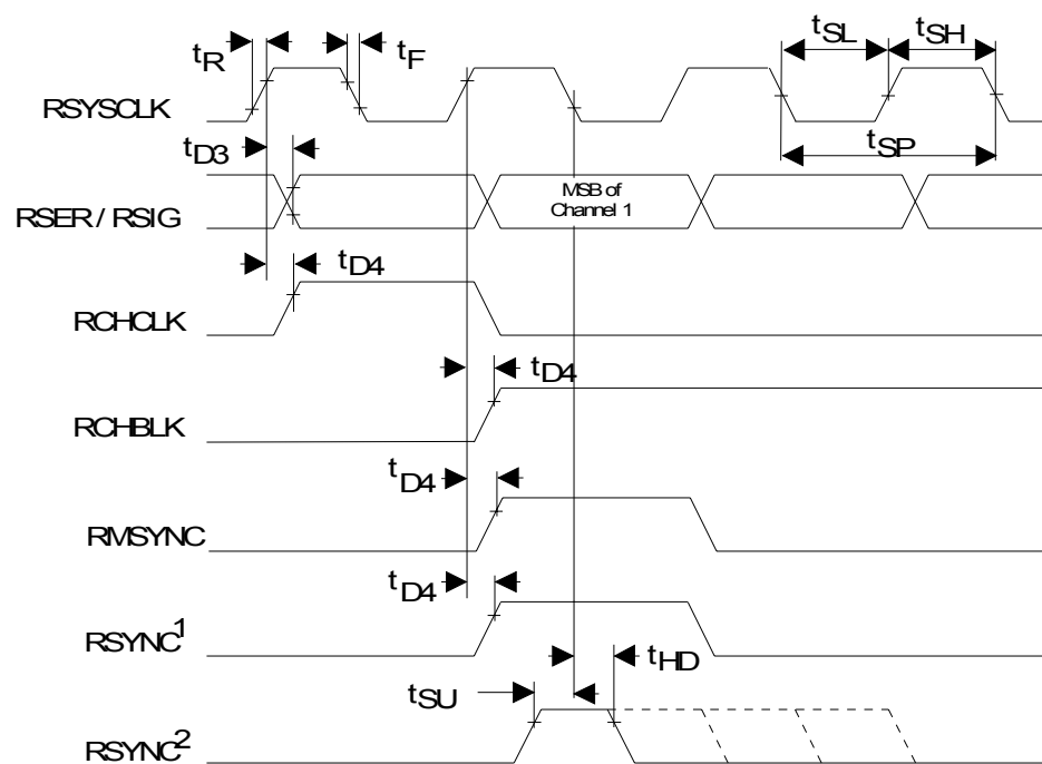
Figure 23-9. RECEIVE SYSTEM SIDE AC TIMING
