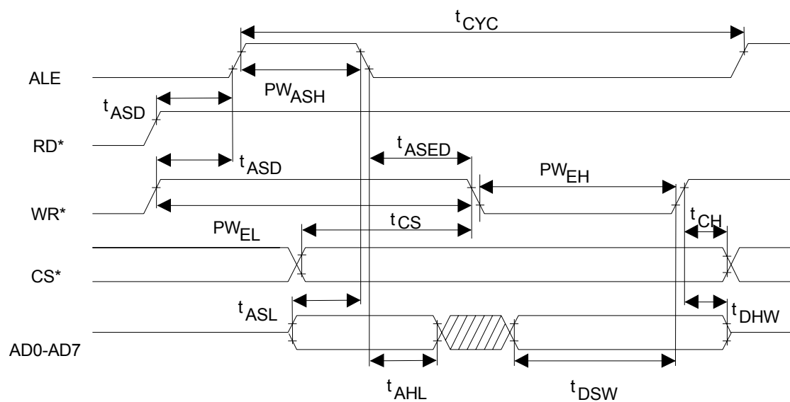
Figure 23-2. INTEL BUS WRITE TIMING (BTS = 0 / MUX = 1)
