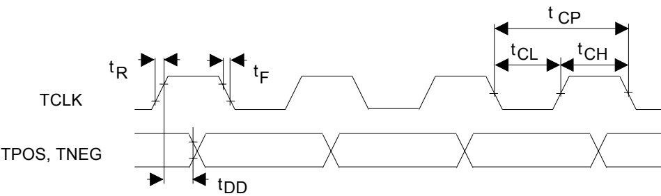
Figure 23-13. TRANSMIT LINE INTERFACE SIDE AC TIMING
