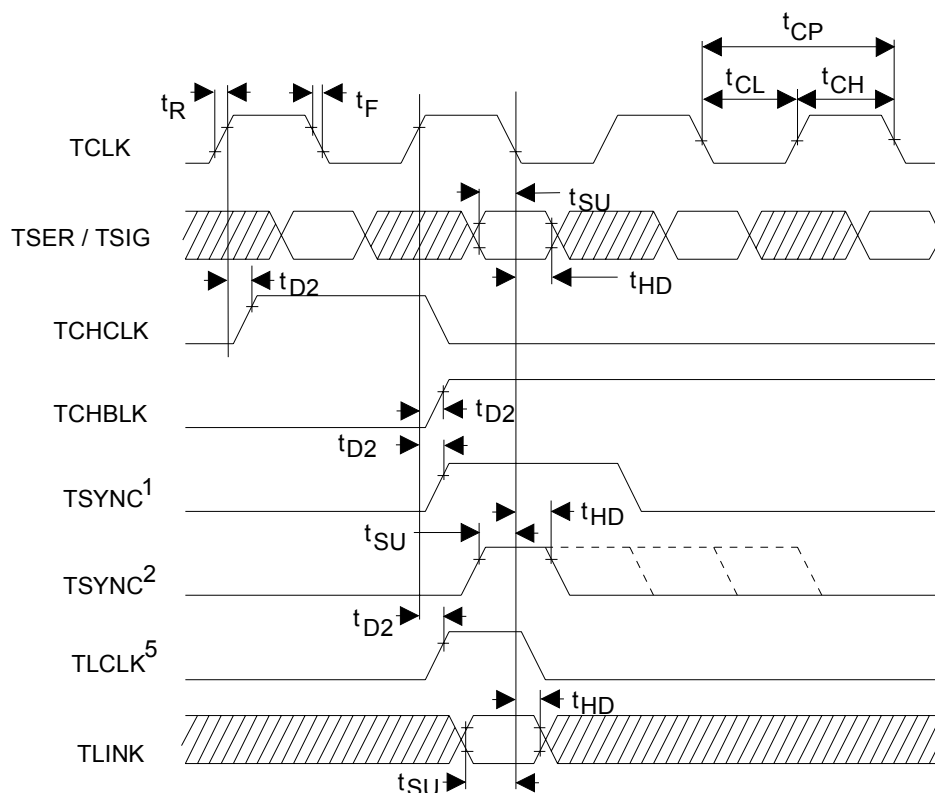
Figure 23-11. TRANSMIT SIDE AC TIMING
