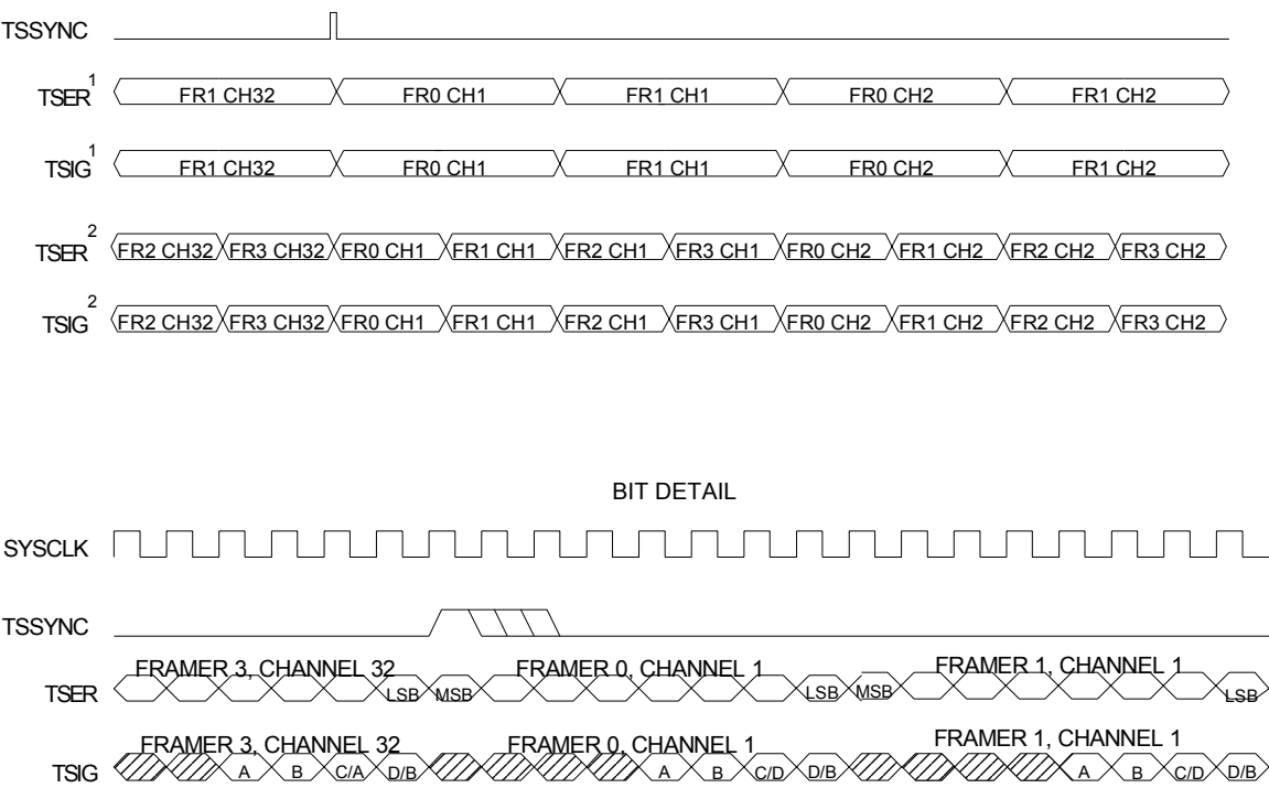
Figure 22-12. TRANSMIT SIDE, INTERLEAVED BUS OPERATION BYTE MODE TIMING
