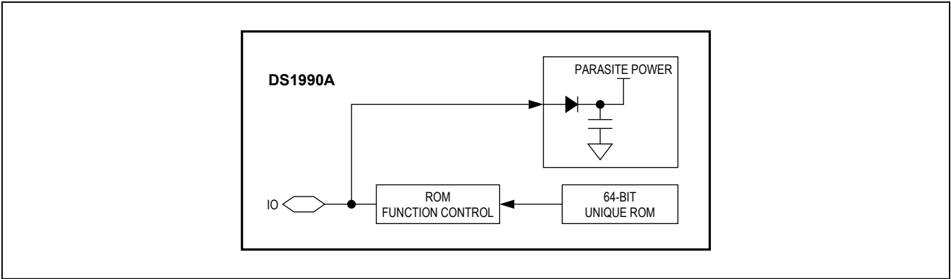
Figure 1. Block Diagram
