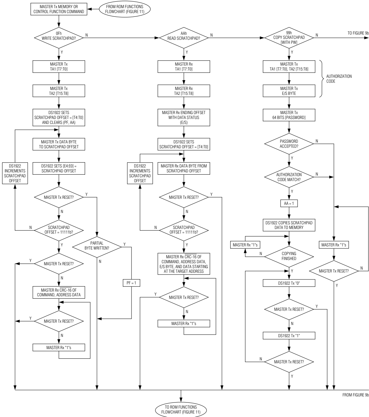
Figure 9a. Memory/Control Function Flowchart
