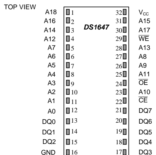
32-Pin Encapsulated DIP Package (32 Pin 740)
