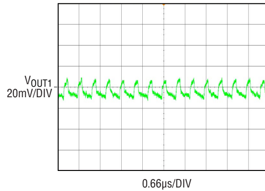
(a) CH1: V_{IN} = 12V , V_{OUT1} = 3.3V , I_{OUT1} = 10A
