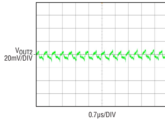
(b) CH2: V_{IN} = 12V , V_{OUT2} = 5V , I_{OUT2} = 7A
