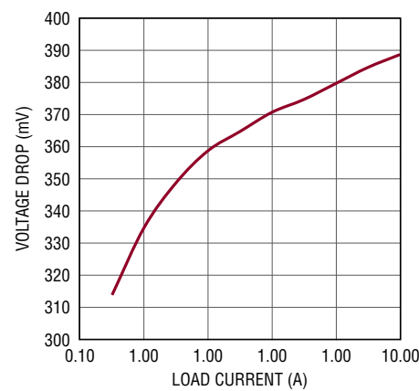
Figure 6. CH3 Voltage Drop in Pass-through Mode ( V_{IN} = 12V )
