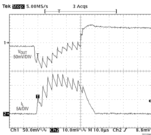
Figure 4b. Load Step Response with Burst Mode Operation Enabled
