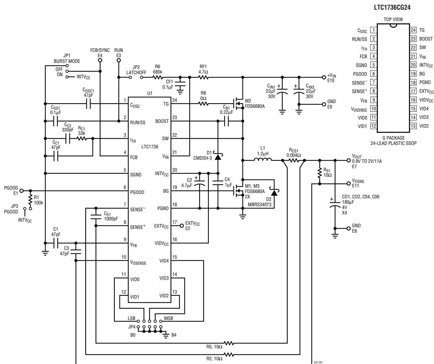
Figure 1. Demo Board Schematic
