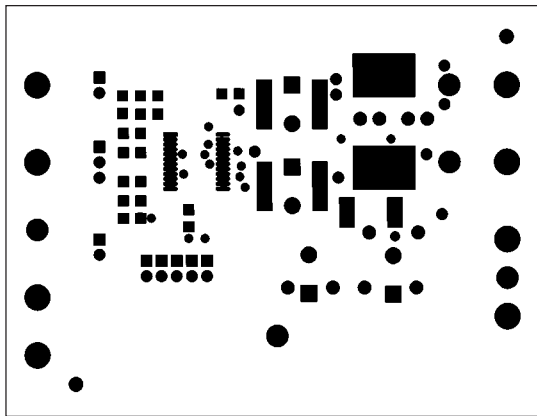
Component Paste Mask
