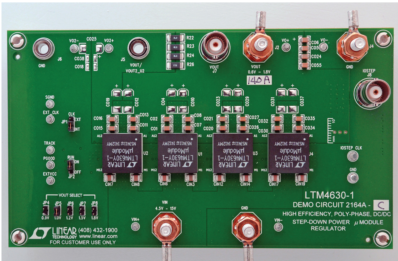
Figure 1. 140A PolyPhase LTM4630-1/DC2164A-C Demo Board
