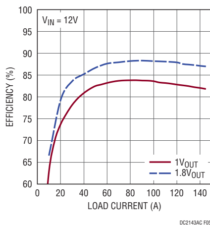
Figure 5. Efficiency vs Load Current at V_{OUT} = 1V and V_{OUT} = 1.8V , f_{SW} = 500kHz
