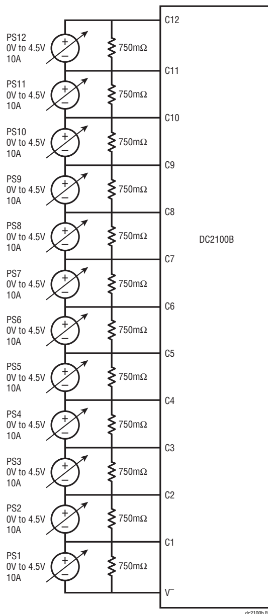
Figure 5. Battery Emulator Concept. Resistors Are Sized to Sink Up to 4.3A at 3.2V
