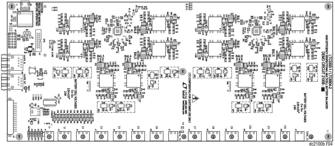
Figure 4. DC2100B-C Demo Board Size Equals 5.5" x 12.8"
