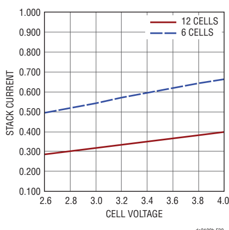
Figure 30. Stack Charge Current
