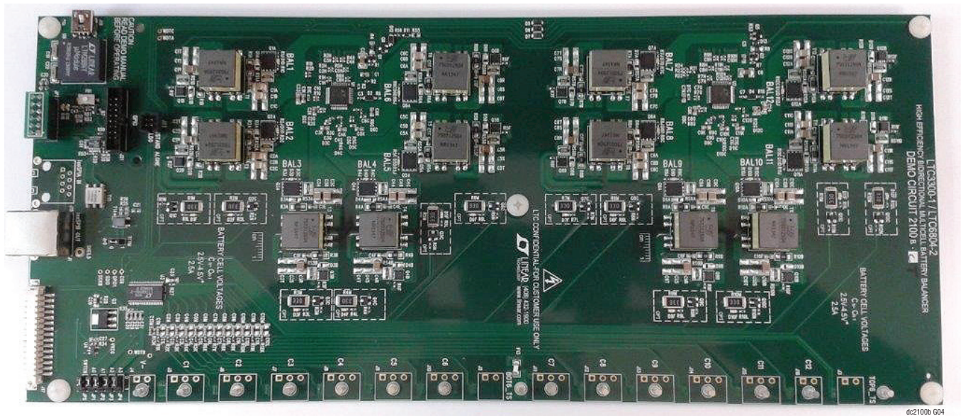
Figure 3. DC2100B-C Demo Board Photo
