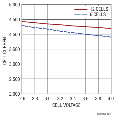
Figure 27. Cell Discharge Current
