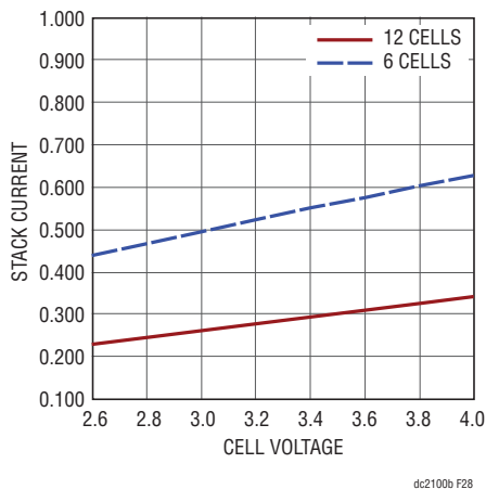
Figure 28. Stack Discharge Current
