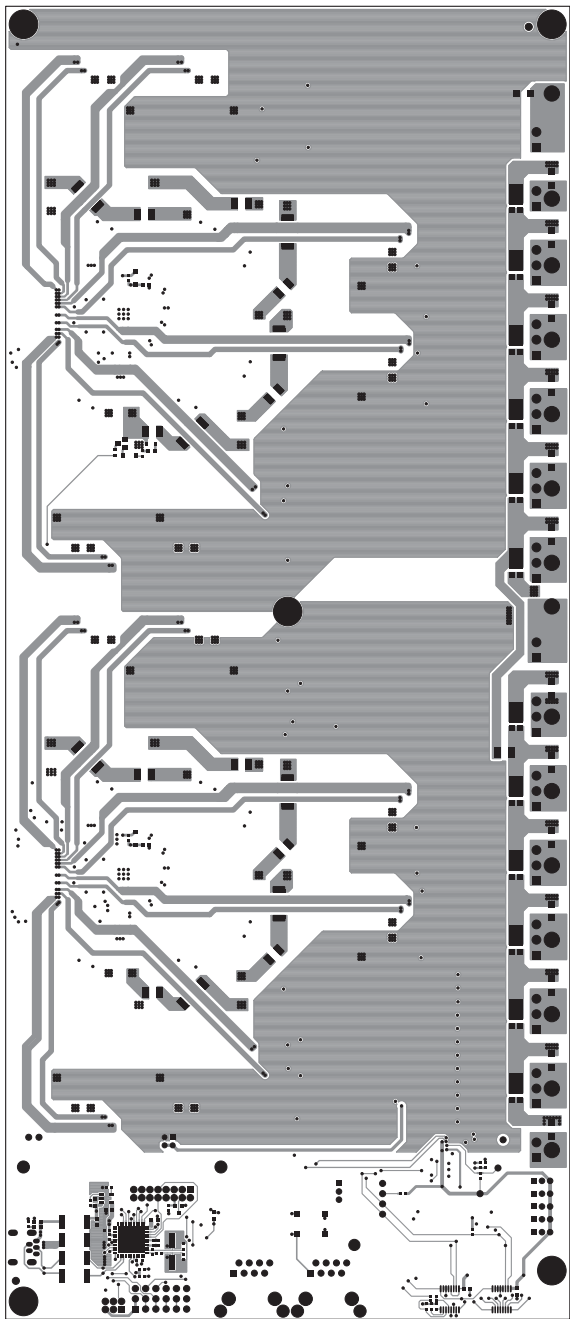
LAYER 4 – BOTTOM SIDE-TOP6/BOT6 PLANE LINEAR TECHNOLOGY DEMO CIRCUIT 2100B-1-A/D• LTC3300-1/LTC6804-2 HIGH EFFICIENCY BIDIRECTIONAL MULTICELL BATTERY BALANCER 02-25-15
