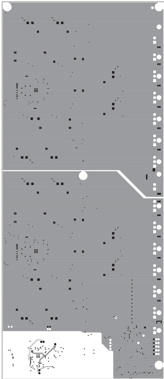
LAYER 3 – V-/C6 GND PLANE LINEAR TECHNOLOGY DEMO CIRCUIT 2100B-1-A/D• LTC3300-1/LTC6804-2 HIGH EFFICIENCY BIDIRECTIONAL MULTICELL BATTERY BALANCER 02-25-15
