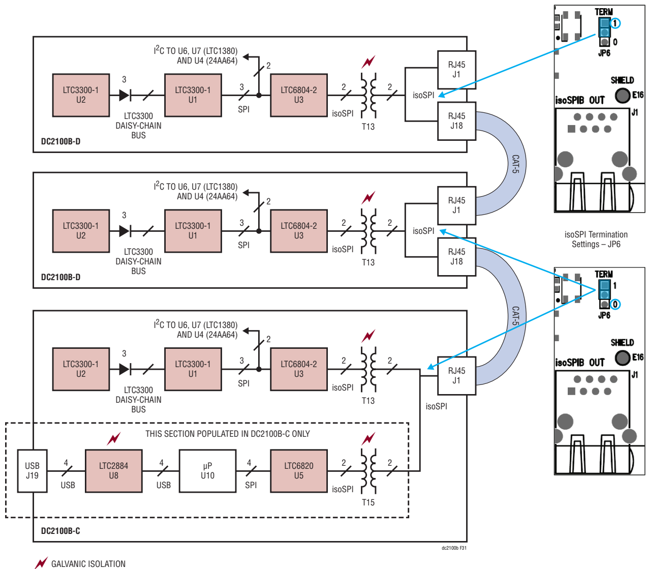
Figure 31. Connection of Multiple DC2100B to Support a Larger Battery Stack
