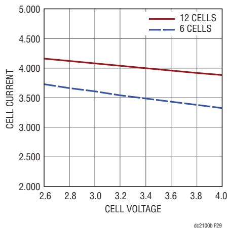
Figure 29. Cell Charge Current
