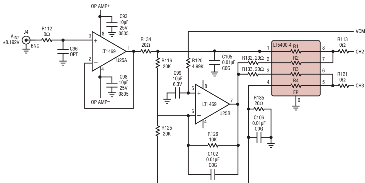
Figure 3. \pm 8.192V Single-Ended to Differential DC Coupled Driver
