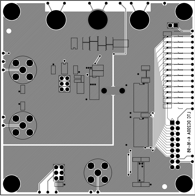
Solder Side
