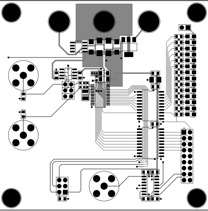
Component Side
