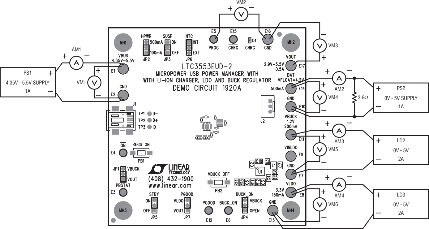
Figure 1. Proper Measurement Equipment Setup for DC1920A
