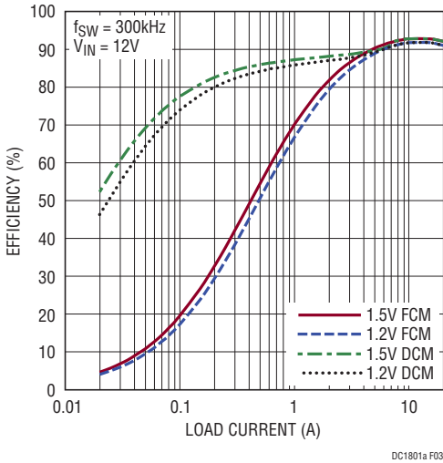
Figure 3. Efficiency Curves for the DC1801A-A ( DCR_{SENSE} ) in FCM and DCM.
