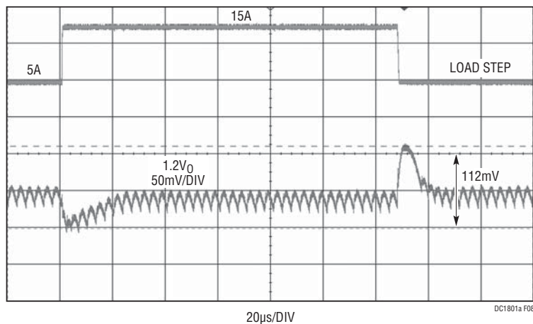
Figure 8. Load Step Response of the 1.2V Rail on the DC1801A-B ( R_{SENSE} ) at V_{IN} = 12V . C_{OUT} = 2 \times Sanyo 2R5TPE330M9 \parallel 2 \times 100\mu F X5R 6.3V 1206, f_{SW} = 300kHz , L = 0.44\mu H , f_{SW} = 300kHz
