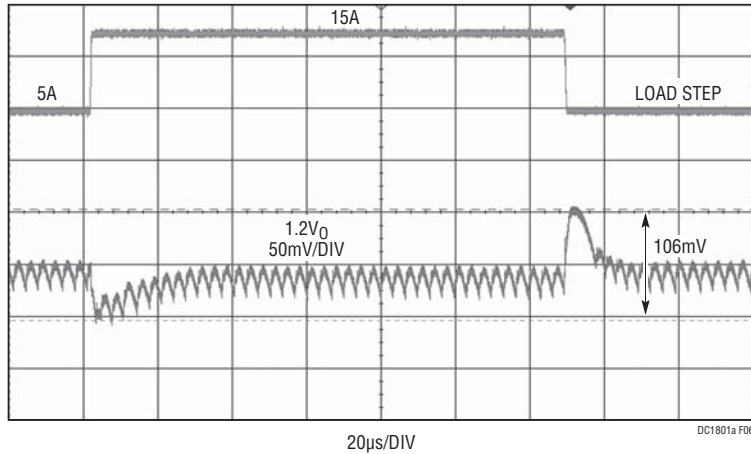
Figure 6. Load Step Response of the 1.2V Rail on the DC1801A-A (DCR SENSE ) at V_{IN} = 12V . C_{OUT} = 2 \times Sanyo 2R5TPE330M9 || 2 \times 100\mu F X5R 6.3V 1206, L = 0.47\mu H , f_{SW} = 300kHz
