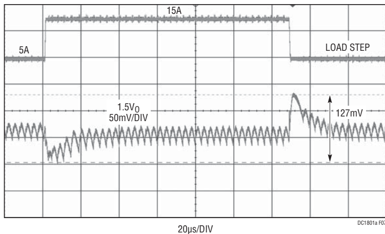
Figure 7. Load Step Response of the 1.5V Rail on the DC1801A-A (DCR SENSE ) at V_{IN} = 12V . C_{OUT} = 2 \times Sanyo 2R5TPE330M9 || 2 \times 100\mu F X5R 6.3V 1206, L = 0.47\mu H , f_{SW} = 300kHz
