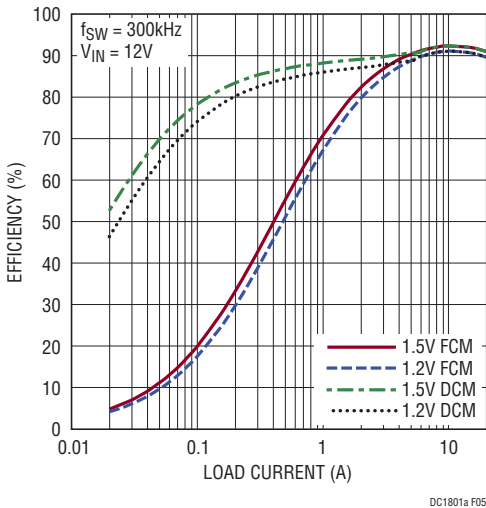
Figure 5. Efficiency Curves for the DC1801A-B ( R_{SENSE} ) in FCM and DCM
