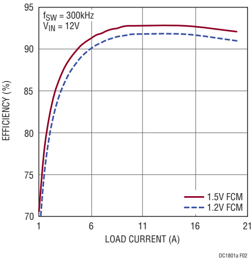
Figure 2. Efficiency Curves for the DC1801A-A ( DCR_{SENSE} ) in FCM
