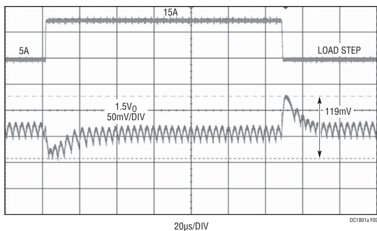
Figure 9. Load Step Response of the 1.5V Rail on the DC1801A-B ( R_{SENSE} ) at V_{IN} = 12V . C_{OUT} = 2 \times Sanyo 2R5TPE330M9 \parallel 2 \times 100\mu F X5R 6.3V 1206, f_{SW} = 300kHz , L = 0.44\mu H , f_{SW} = 300kHz
