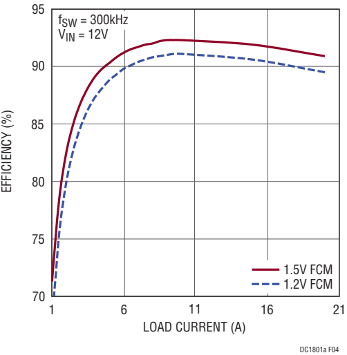
Figure 4. Efficiency Curves for the DC1801A-B ( R_{SENSE} ) in FCM
