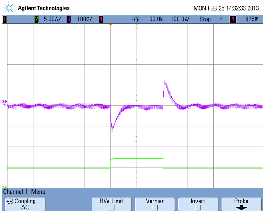
Figure 4. Transient Response Waveform at 24V IN and 5A – 7.5A – 5A OUT (5A, 100mV, 100 \mu s/Div)
