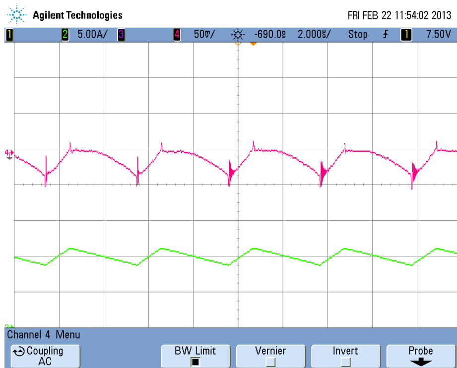
Figure 3. Output Ripple at 24V IN and 10A OUT (50mV, 5A, 2 \mu s/Div, 20MHz)
