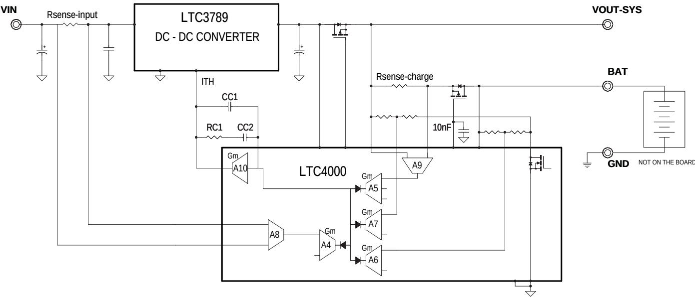
Figure 4. Block Diagram
