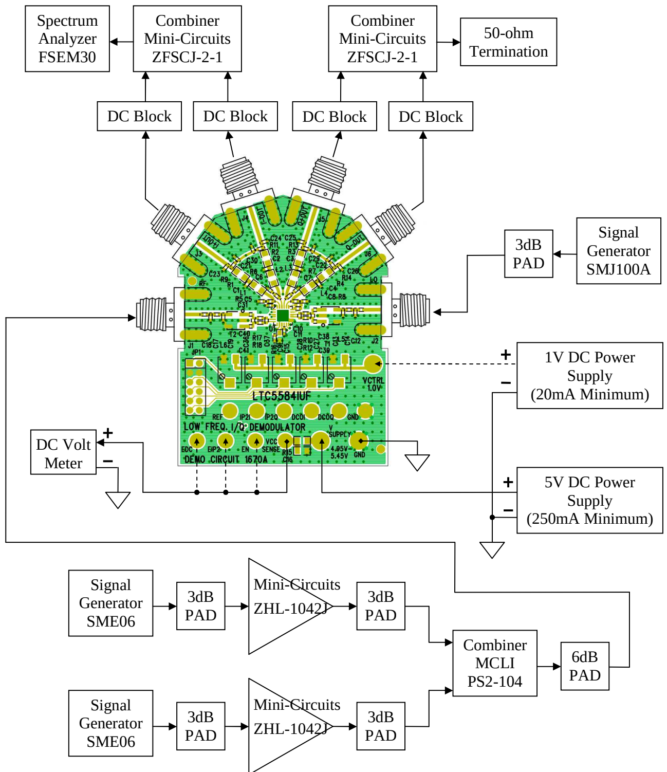
Figure 1. Measurement Setup
