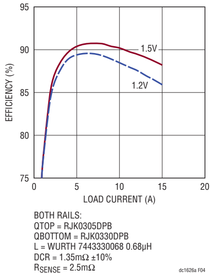
Figure 4. Efficiency Curves for the DC1626A-B (RSENSE) in FCM
