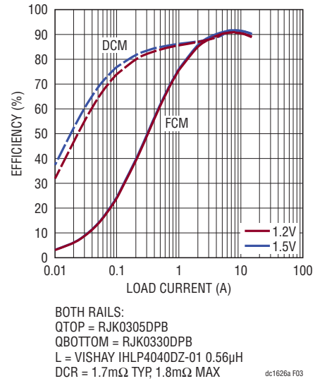
Figure 3. Efficiency Curves for the DC1626A-A (DCR Sense) in FCM and DCM.
