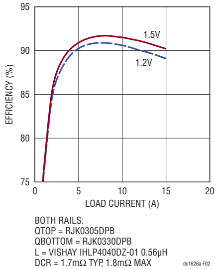
Figure 2. Efficiency Curves for the DC1626A-A (DCR Sense) in FCM
