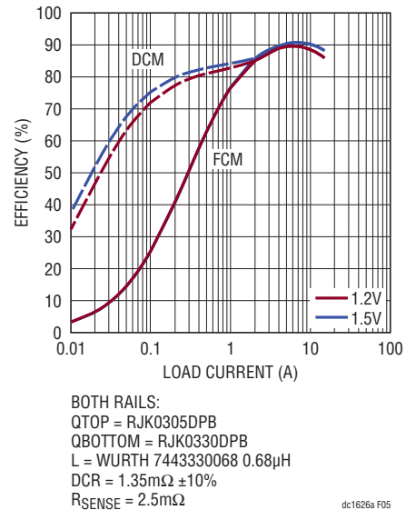
Figure 5. Efficiency Curves for the DC1626A-B (RSENSE) in FCM and DCM
