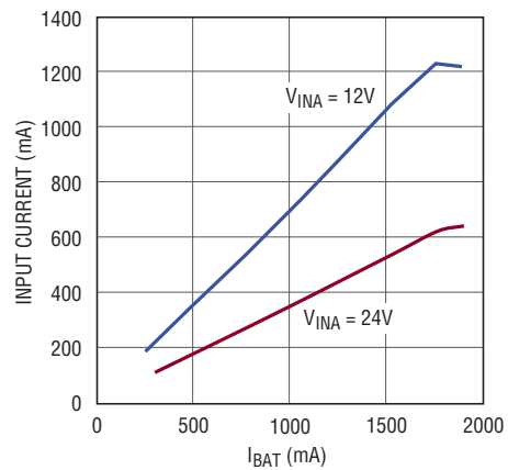
Figure 3. Input Current vs I_{BAT} , 7.2V Float
