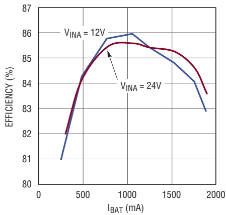
Figure 2. Efficiency vs I_{BAT} , 7.2V Float
