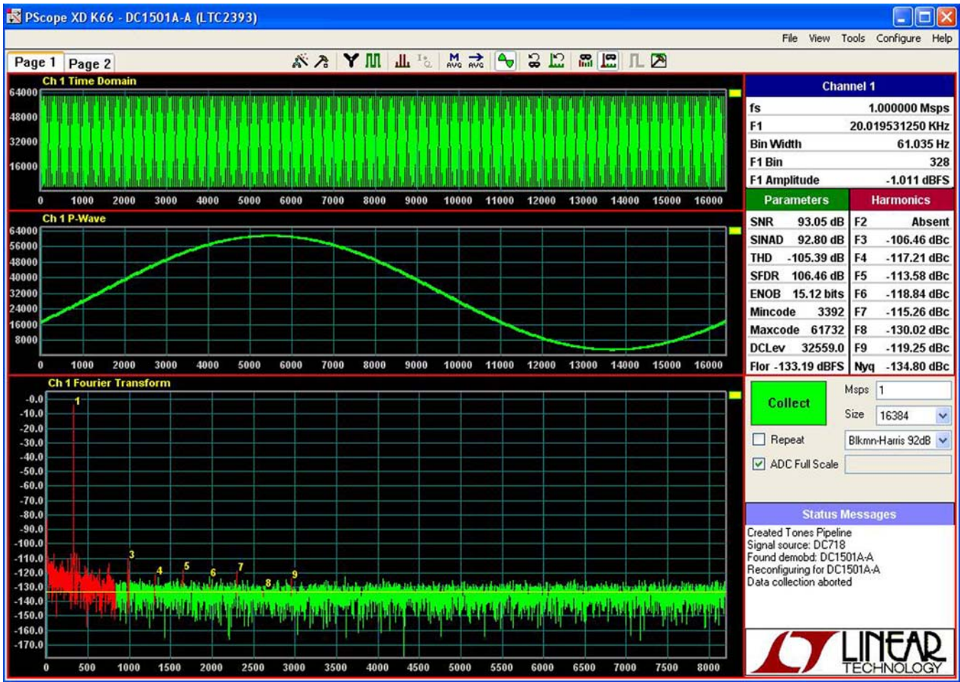
Figure 6. DC1501A FastDAACS Screenshot
