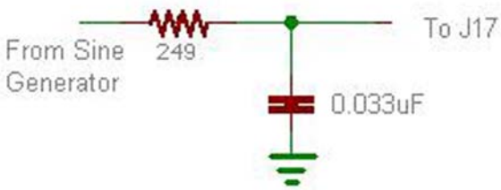
Figure 5. 20kHz RC filter
