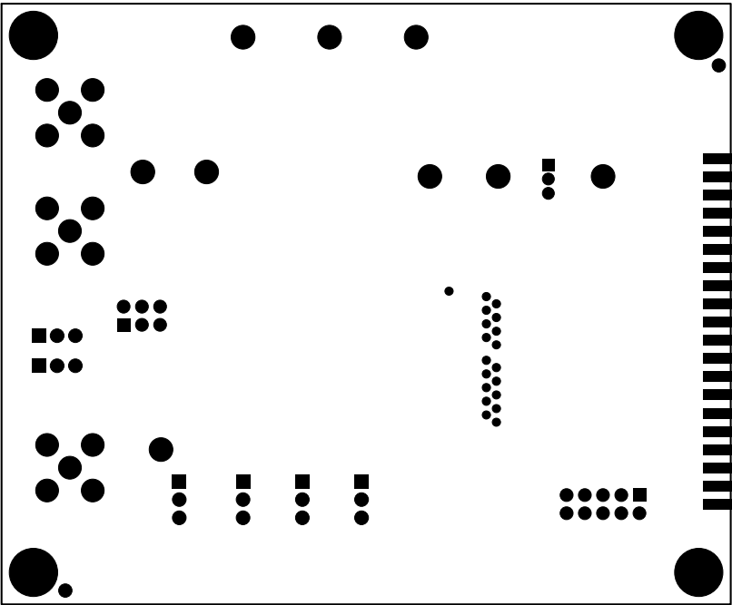
Bottom Solder Mask
