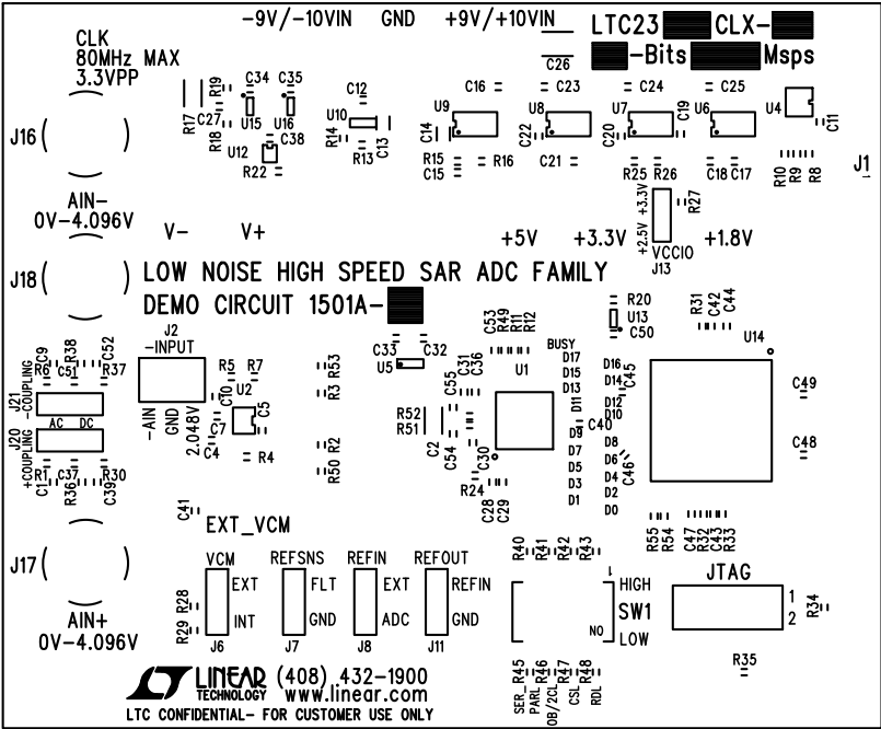
Top Silkscreen
