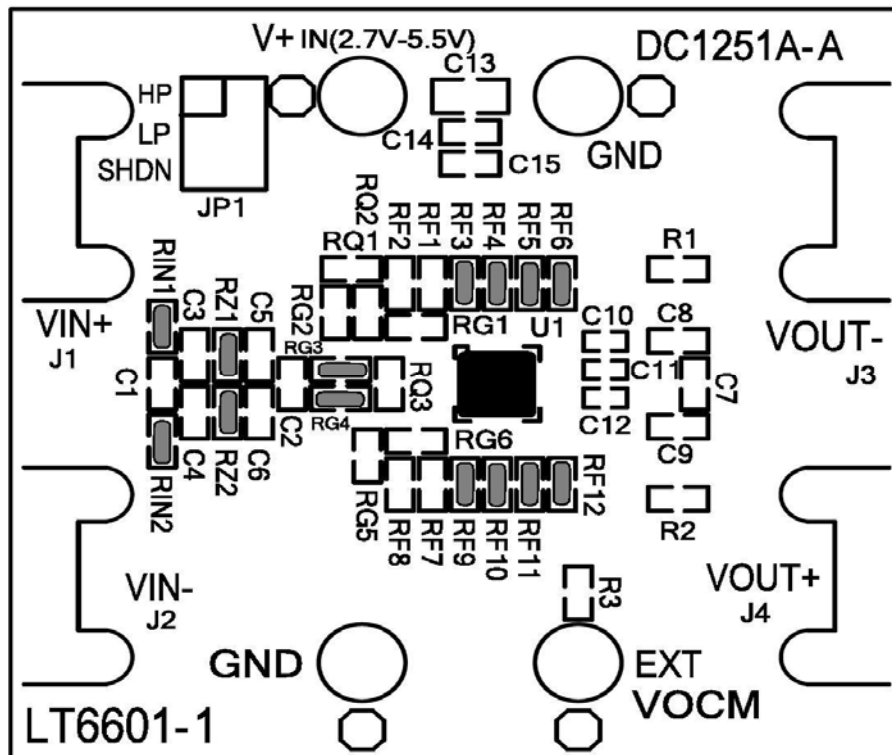
DC1251A TOP SILK SCREEN
