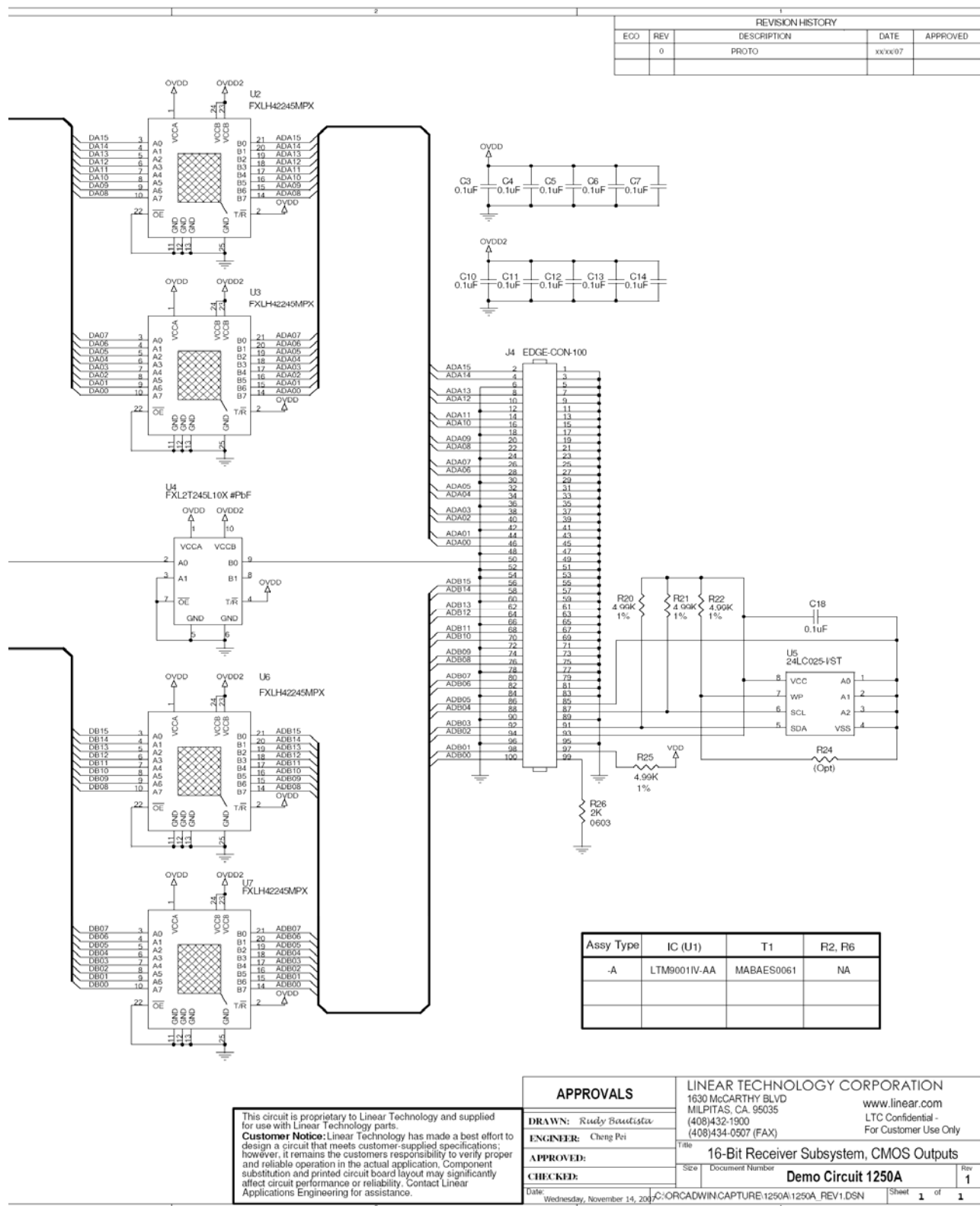
DC1250 Schematic (Separated into 2 pages)
