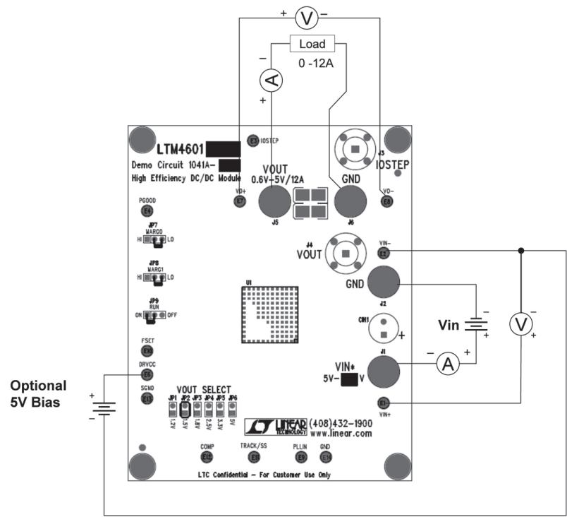
Figure 1. Demo Board Setup
