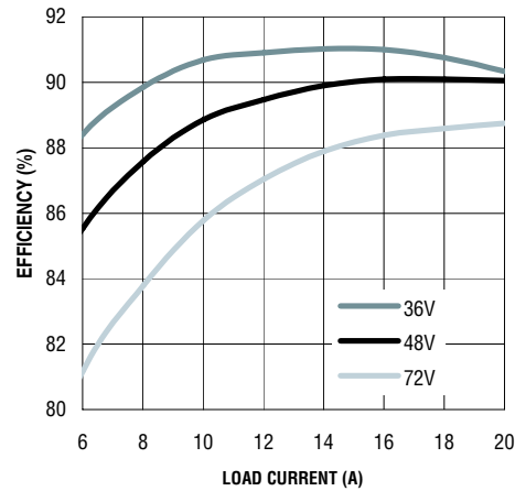
Figure 3. Efficiency (200l/m airflow)
