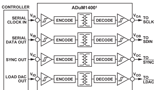
Figure 53. Isolated Interface
