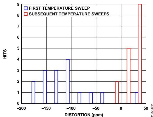
Figure 49. Thermal Hysteresis
