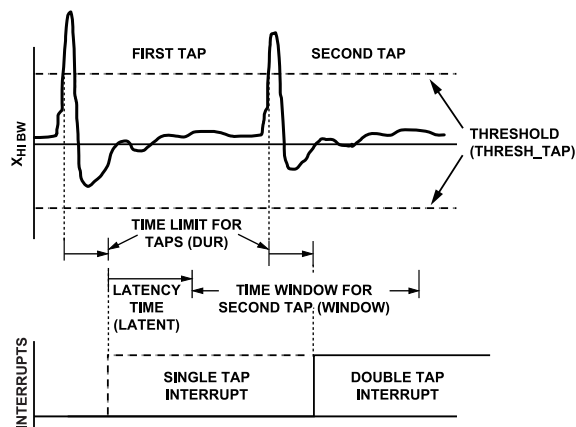
Figure 49. Tap Interrupt Function with Valid Single and Double Taps
