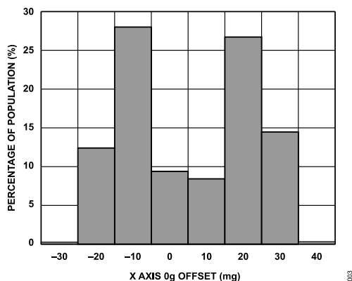
Figure 18. X-Axis Zero g Offset at 25^\circ\text{C} , V_S = 2\text{ V}
