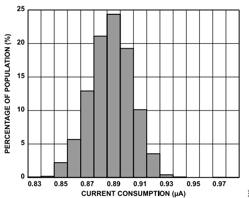
Figure 34. Current Consumption at 25°C, Normal Mode, ODR = 100 Hz, V_S = 2 V
