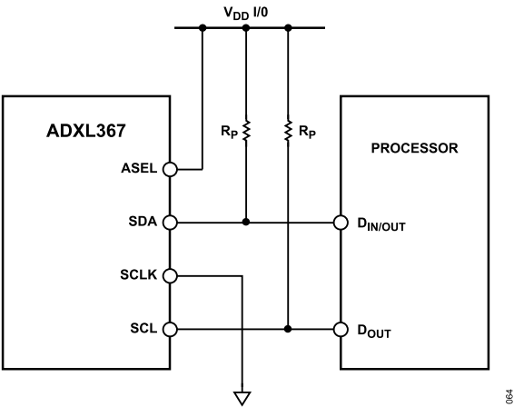
Figure 53. I 2 C Connection Diagram (Address 0x53)
