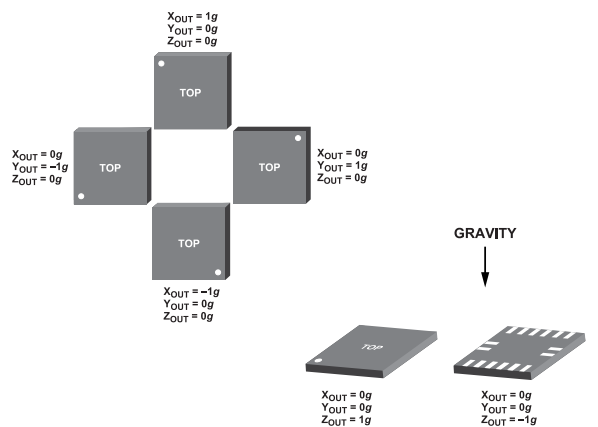
Figure 66. Output Response vs. Orientation to Gravity
