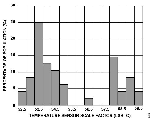
Figure 38. Temperature Sensor Scale Factor, V_S = 2\text{ V}
