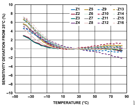
Figure 32. Sensitivity Deviation from 25°C vs. Temperature, 16 ADXL367 Devices Soldered to PCB, ODR = 100 Hz, V_S = 2 V, Z-Axis
