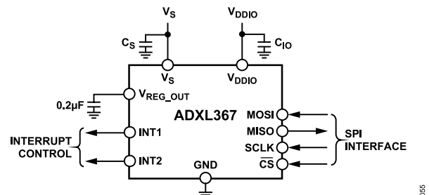
Figure 60. Recommended Bypass Capacitors
