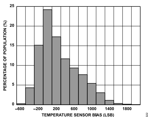
Figure 37. Temperature Sensor Response at 25°C, V_S = 2\text{ V}
