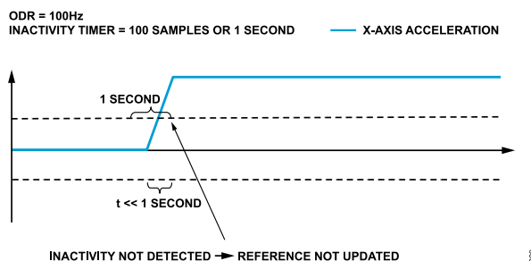
Figure 45. Referenced Inactivity Thresholds, Fast Change in Acceleration
