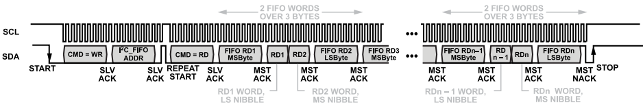
Figure 14. I2C FIFO Read (N 12-Bit Words)
