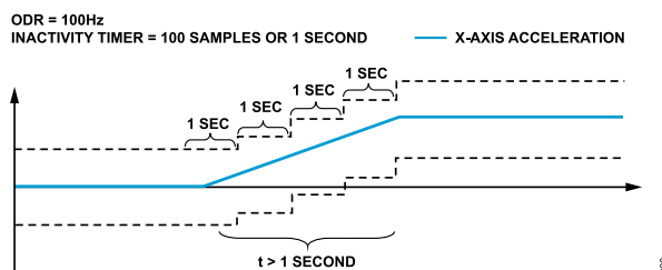
Figure 44. Referenced Inactivity Thresholds, Slow Change in Acceleration
