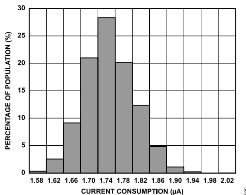
Figure 35. Current Consumption at 25°C, Low Noise Mode, ODR = 100 Hz, V_S = 2 V
