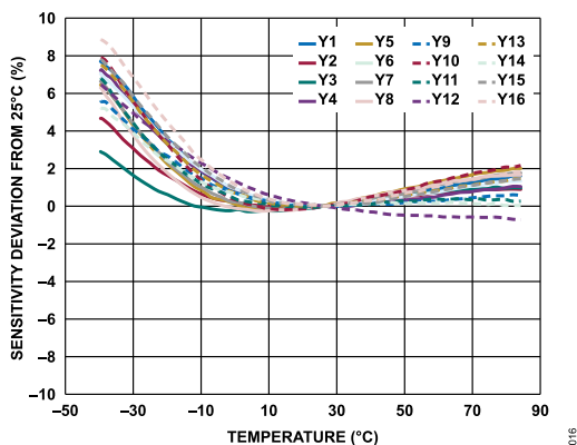
Figure 31. Sensitivity Deviation from 25°C vs. Temperature, 16 ADXL367 Devices Soldered to PCB, ODR = 100 Hz, V_S = 2 V, Y-Axis
