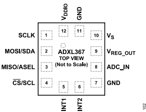
Figure 17. Pin Configuration
