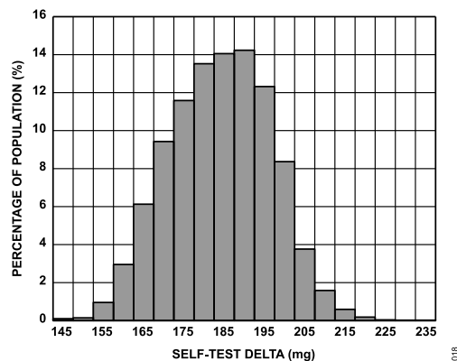
Figure 33. X-Axis Self Test Response at 25°C, V_S = 2 V
