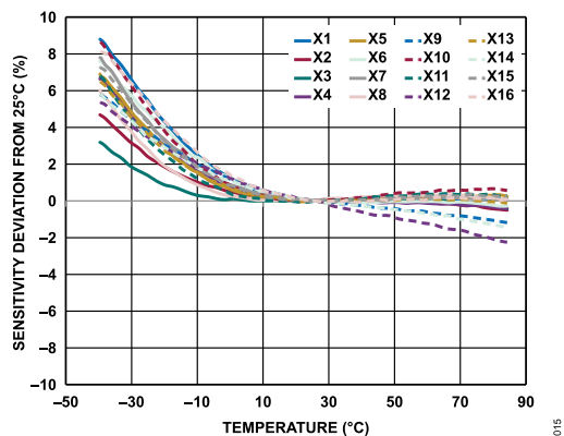
Figure 30. Sensitivity Deviation from 25°C vs. Temperature, 16 ADXL367 Devices Soldered to PCB, ODR = 100 Hz, V_S = 2 V, X-Axis
