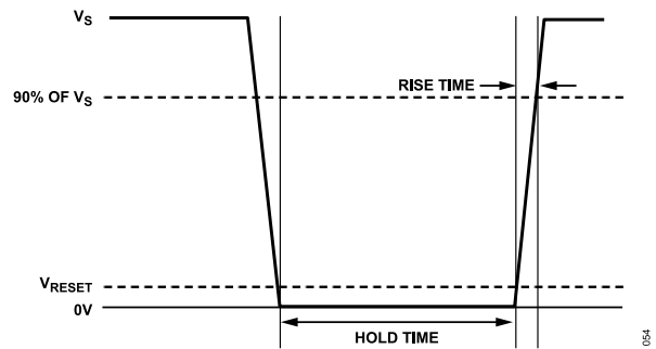
Figure 59. Power Supply Reset and Start-Up Requirements
