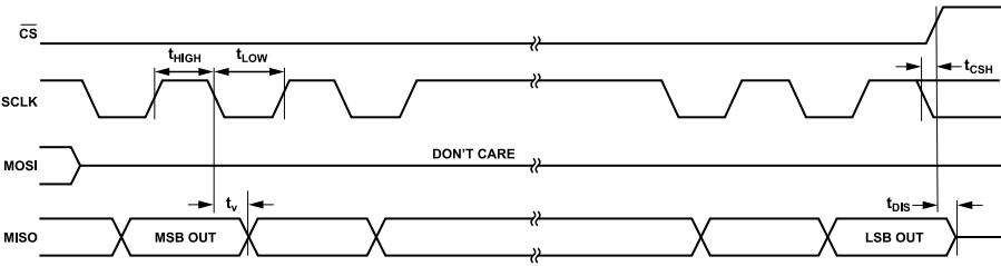
Figure 11. Timing Diagram for SPI Send Instructions
