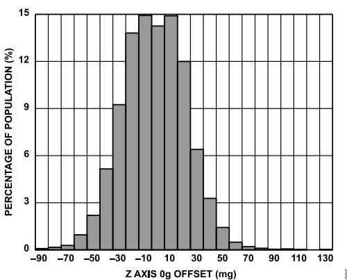
Figure 20. Z-Axis Zero g Offset at 25^\circ\text{C} , V_S = 2\text{ V}
