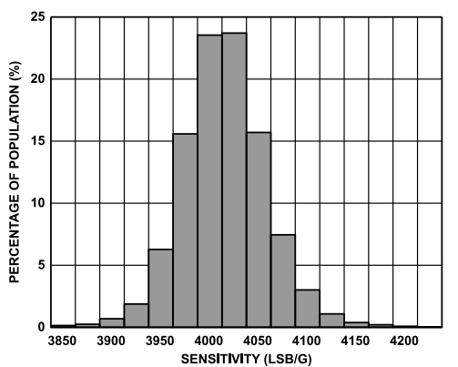
Figure 23. Z-Axis Sensitivity at 25^\circ\text{C} , V_S = 2\text{ V} , \pm 2\text{ g} Range
