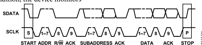
Figure 10. Bus Data Transfer
