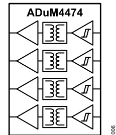
Figure 6. ADuM4474
