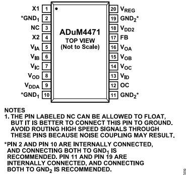
Figure 9. ADuM4471 Pin Configuration
