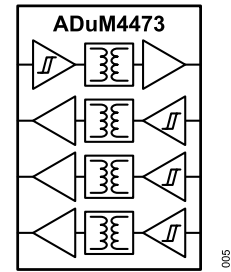
Figure 5. ADuM4473
