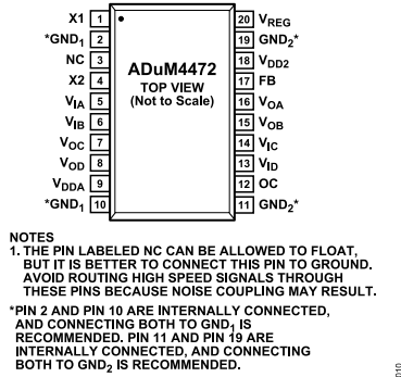
Figure 10. ADuM4472 Pin Configuration
