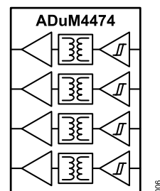
Figure 6. ADuM4474
