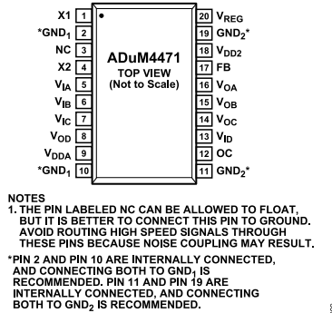
Figure 9. ADuM4471 Pin Configuration
