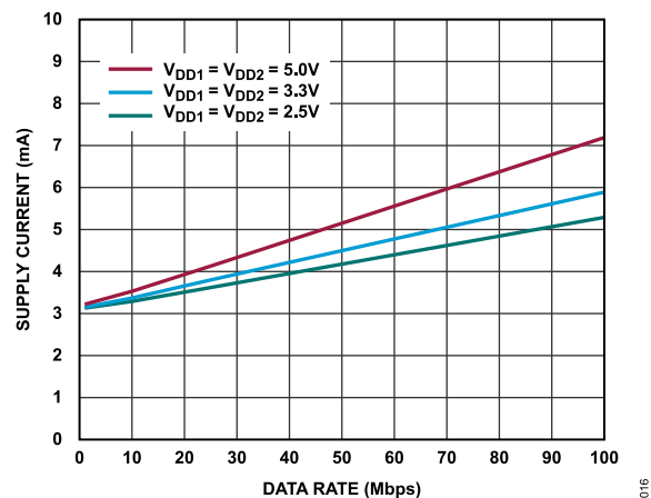
Figure 13. ADuM342E I_{DD2} Supply Current vs. Data Rate at Various Voltages
