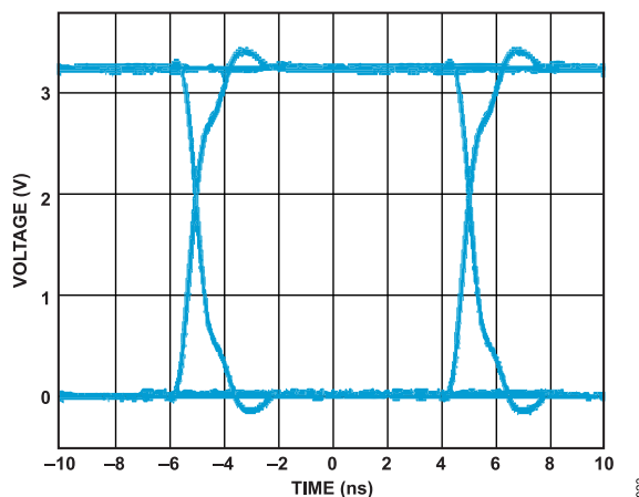
Figure 23. ADuM341E Output Channel Eye Diagram ( V_{DD1} = V_{DD2} = 3.3 \text{ V} , 100 Mbps, T_A = 25^\circ\text{C} , C_L = 15 \text{ pF} , PRBS15 Input)
