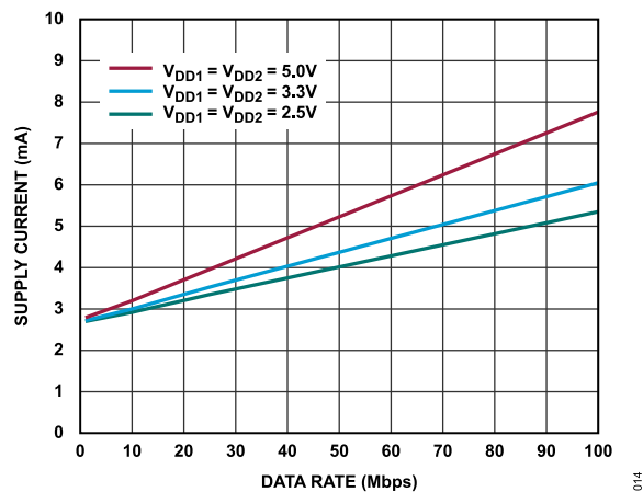
Figure 11. ADuM341E I_{DD2} Supply Current vs. Data Rate at Various Voltages
