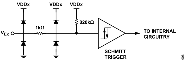
Figure 19. V_{E1} , V_{E2} Input Schematics
