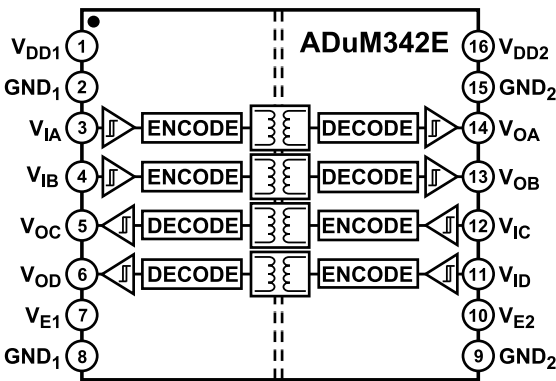
Figure 3. ADuM342E Functional Block Diagram
