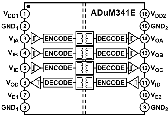
Figure 2. ADuM341E Functional Block Diagram
