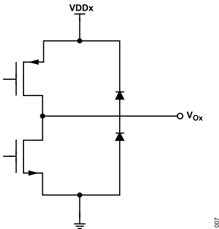
Figure 20. V_{OA} , V_{OB} , V_{OC} , V_{OD} Output Schematics
