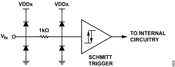
Figure 18. V_{IA} , V_{IB} , V_{IC} , V_{ID} Input Schematics
