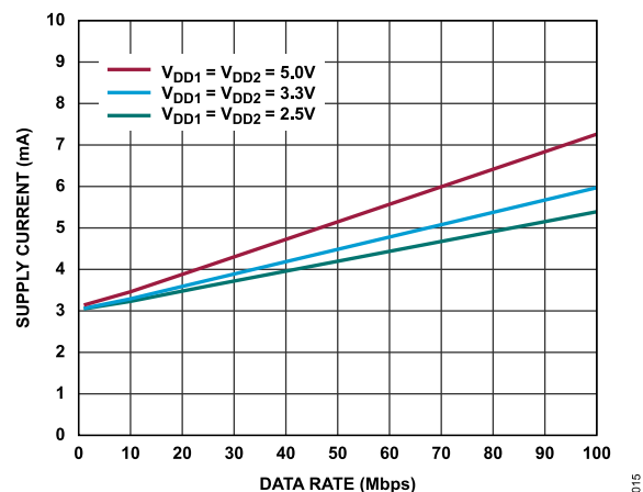
Figure 12. ADuM342E I_{DD1} Supply Current vs. Data Rate at Various Voltages
