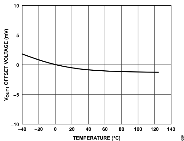
Figure 7. V_{OUT1} Offset Voltage vs. Temperature
