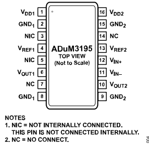
Figure 3. Pin Configuration
