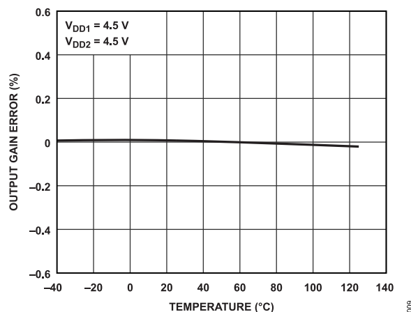
Figure 8. Output Gain Error vs. Temperature
