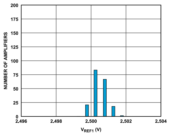
Figure 21. V_{REF1} Distribution at 25°C
