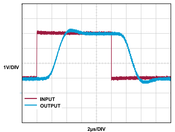
Figure 20. Output Square-Wave Response
