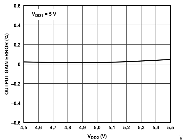
Figure 9. Output Gain Error vs. V_{DD2}
