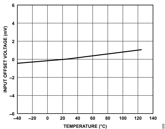
Figure 4. Op Amp Input Offset Voltage vs. Temperature
