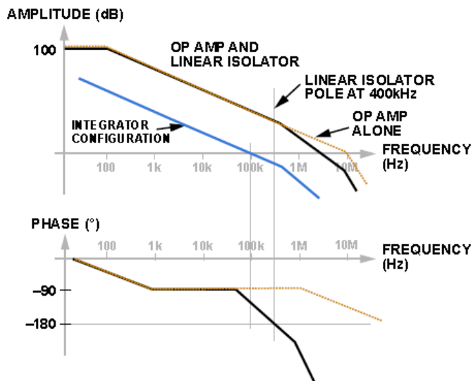
Figure 7. Bode Plot 2
