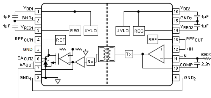
Figure 3. Test Circuit 1: Accuracy Circuit Using EAOUT1
