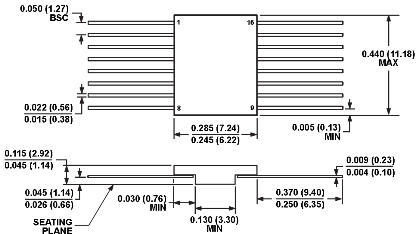
Figure 10. 16-Lead Bottom Brazed Flatpack Dimensions shown in inches and (millimeters)
