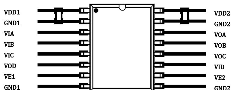
Figure 5 – Recommended Printed Circuit Board Layout
