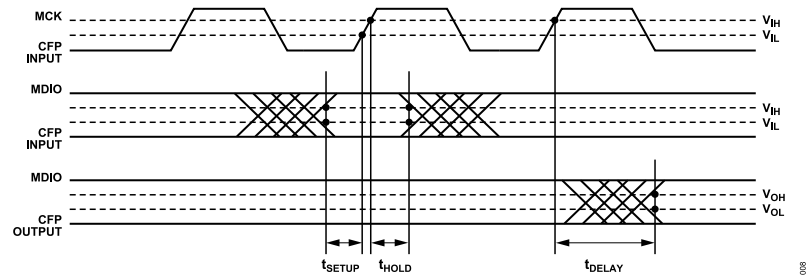
Figure 7. MDIO Timing
