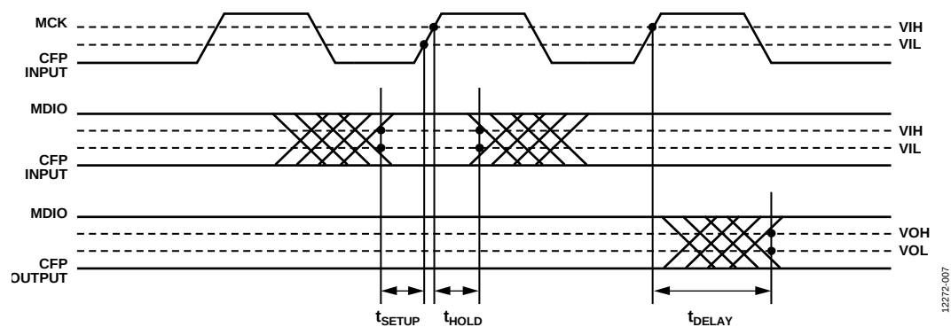
Figure 7. MDIO Timing
