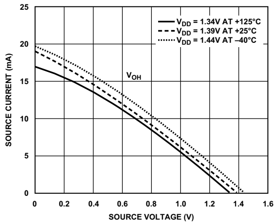
Figure 80. Driver Type B and Driver Type C (DDR3L Drive Strength 60 \Omega )
