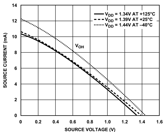
Figure 92. Driver Type B and Driver Type C (DDR3L Drive Strength 100 \Omega )
