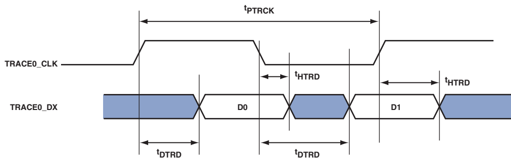
Figure 64. Trace Timing
