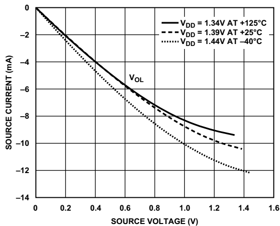
Figure 93. Driver Type B and Driver Type C (DDR3L Drive Strength 100 \Omega )
