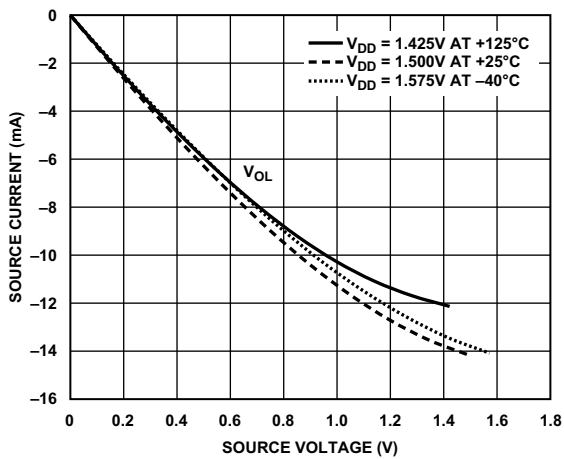
Figure 87. Driver Type B and Driver Type C (DDR3 Drive Strength 90 \Omega )
