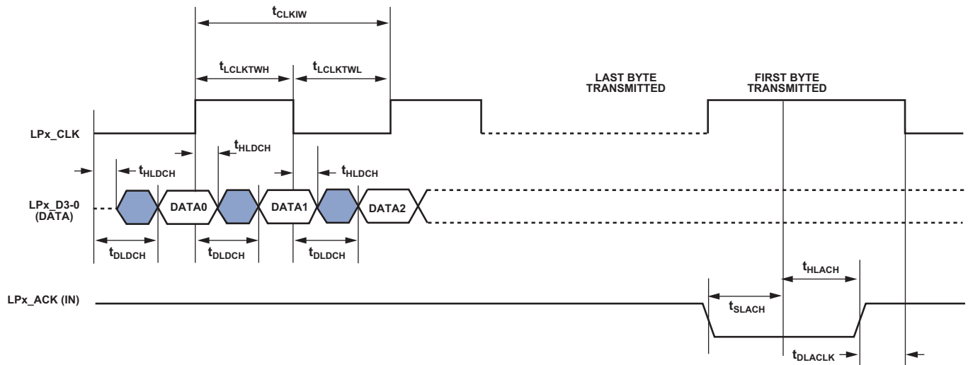
Figure 14. LPs DDR—Transmit
