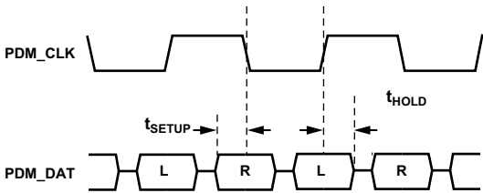
Figure 66. PDM Timing
