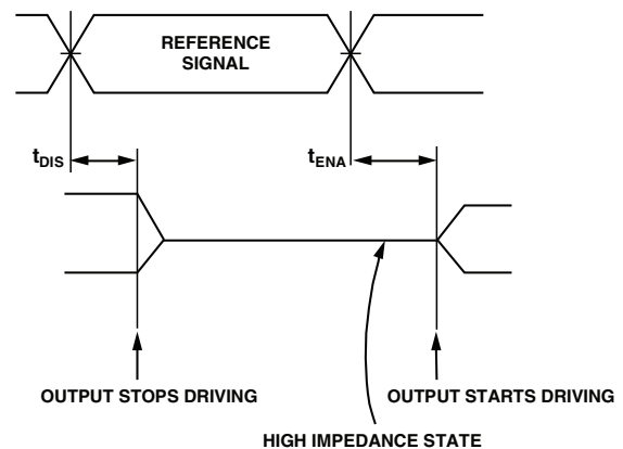
Figure 95. Output Enable/Disable
