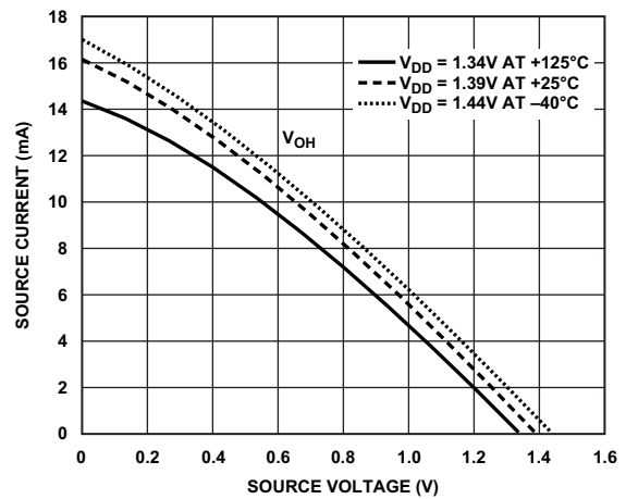
Figure 84. Driver Type B and Driver Type C (DDR3L Drive Strength 70 \Omega )
