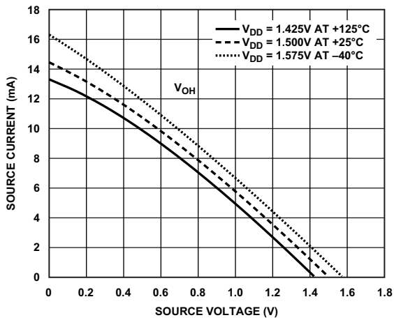
Figure 86. Driver Type B and Driver Type C (DDR3 Drive Strength 90 \Omega )
