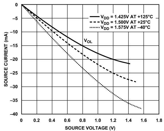
Figure 71. Driver Type B and Driver Type C (DDR3 Drive Strength 40 \Omega )
