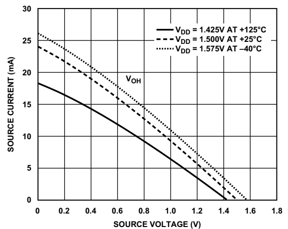
Figure 78. Driver Type B and Driver Type C (DDR3 Drive Strength 60 \Omega )
