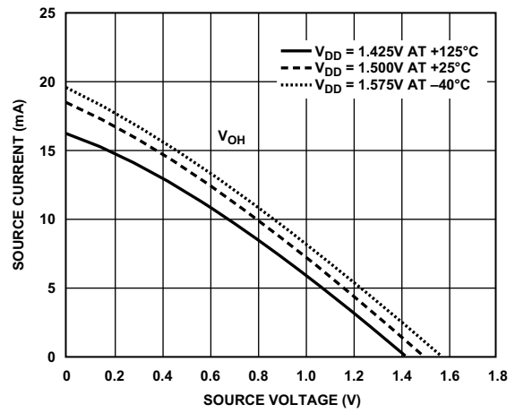
Figure 82. Driver Type B and Driver Type C (DDR3 Drive Strength 70 \Omega )
