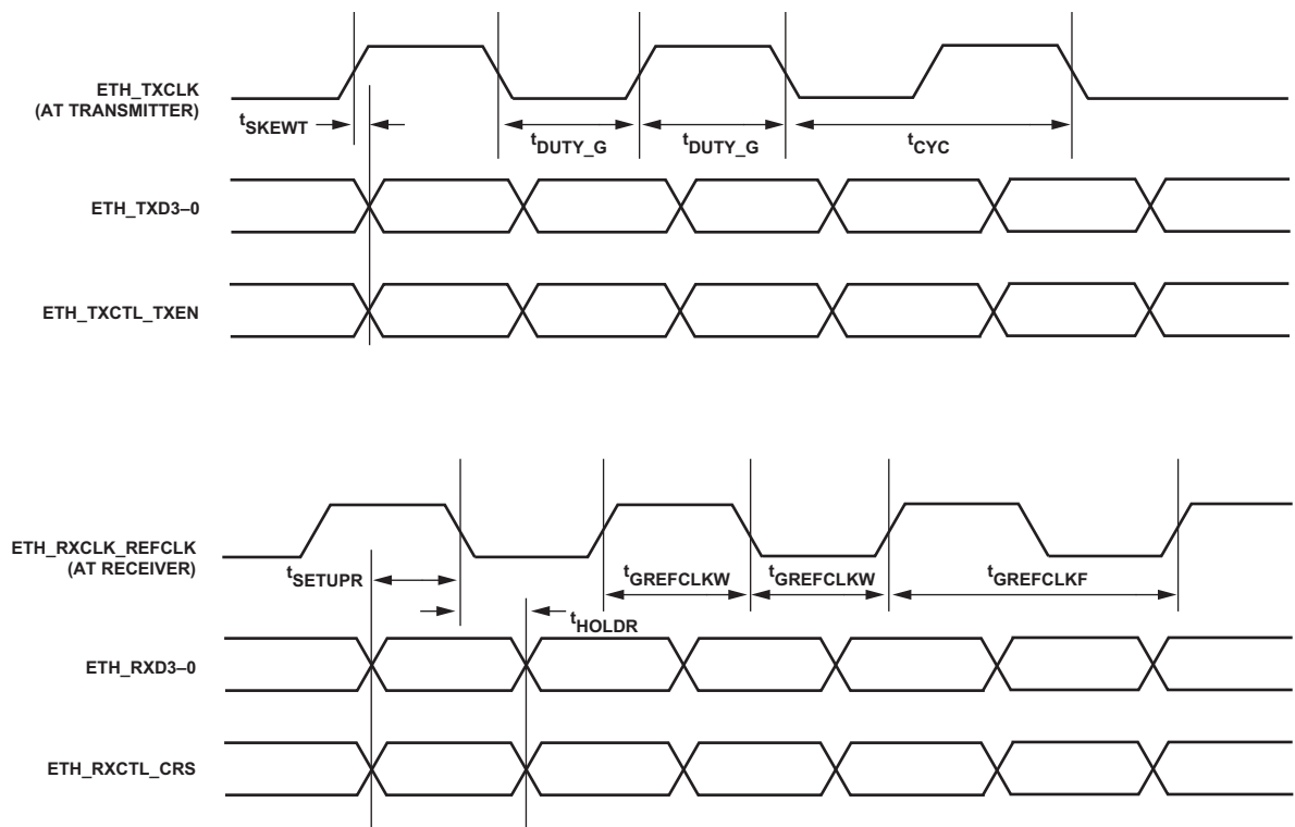
Figure 40. Gigabit EMAC Controller Timing—RGMII
