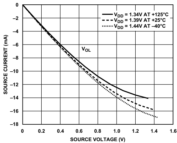
Figure 81. Driver Type B and Driver Type C (DDR3L Drive Strength 60 \Omega )
