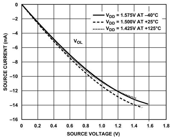
Figure 91. Driver Type B and Driver Type C (DDR3 Drive Strength 100 \Omega )
