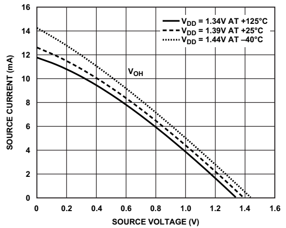
Figure 88. Driver Type B and Driver Type C (DDR3L Drive Strength 90 \Omega )
