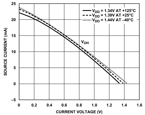
Figure 76. Driver Type B and Driver Type C (DDR3L Drive Strength 50 \Omega )
