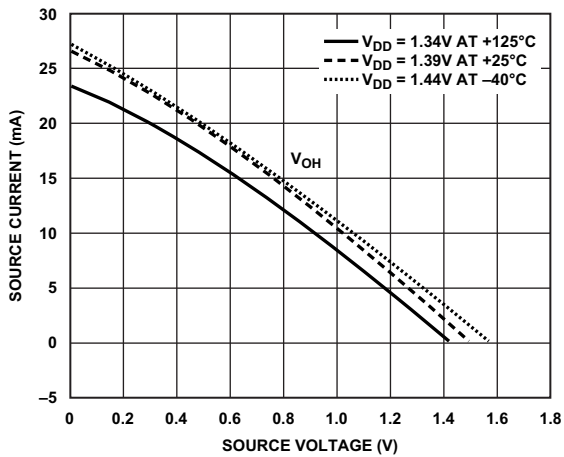
Figure 74. Driver Type B and Driver Type C (DDR3 Drive Strength 50 \Omega )
