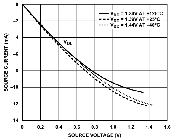
Figure 89. Driver Type B and Driver Type C (DDR3L Drive Strength 90 \Omega )
