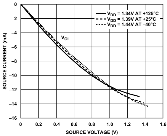
Figure 85. Driver Type B and Driver Type C (DDR3L Drive Strength 70 \Omega )
