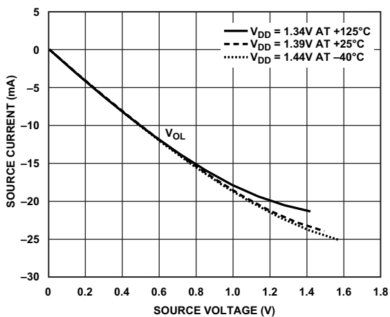
Figure 75. Driver Type B and Driver Type C (DDR3 Drive Strength 50 \Omega )
