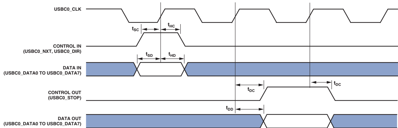
Figure 34. USB Timing
