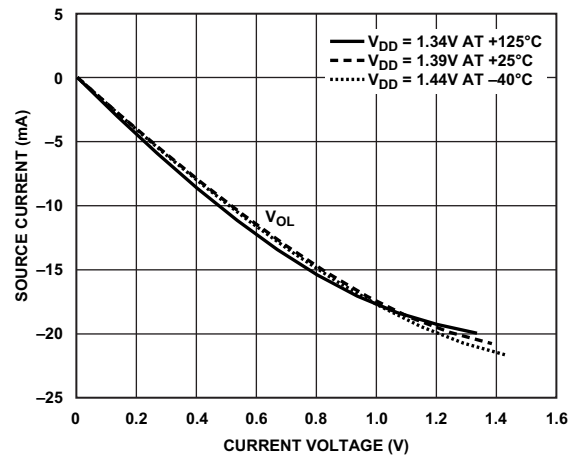
Figure 77. Driver Type B and Driver Type C (DDR3L Drive Strength 50 \Omega )
