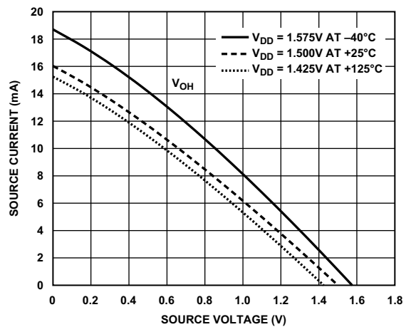
Figure 90. Driver Type B and Driver Type C (DDR3 Drive Strength 100 \Omega )
