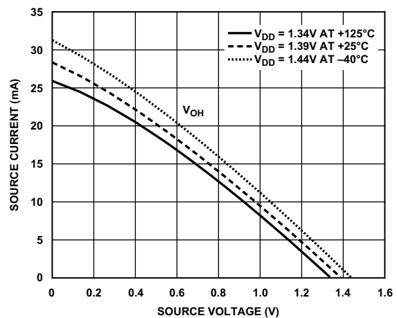
Figure 72. Driver Type B and Driver Type C (DDR3L Drive Strength 40 \Omega )
