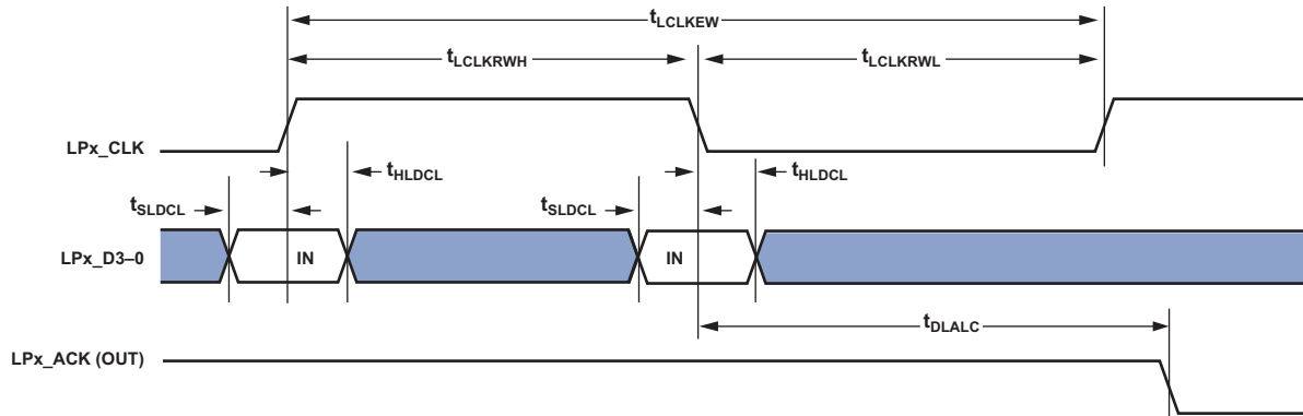
Figure 13. LPs DDR—Receive
