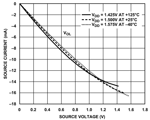
Figure 83. Driver Type B and Driver Type C (DDR3 Drive Strength 70 \Omega )
