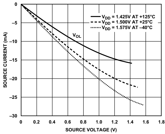
Figure 79. Driver Type B and Driver Type C (DDR3 Drive Strength 60 \Omega )
