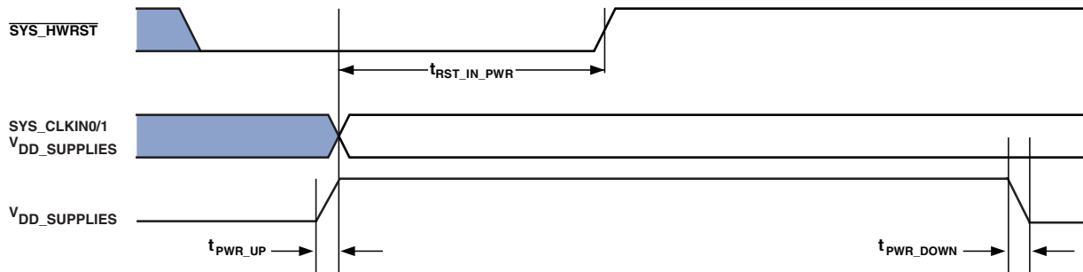
Figure 8. Power-Up Reset Timing
