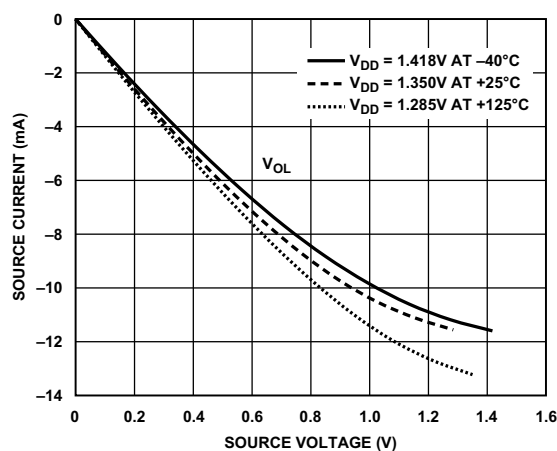
Figure 36. Driver Type B and Driver Type C (DDR3L Drive Strength 100 \Omega )
