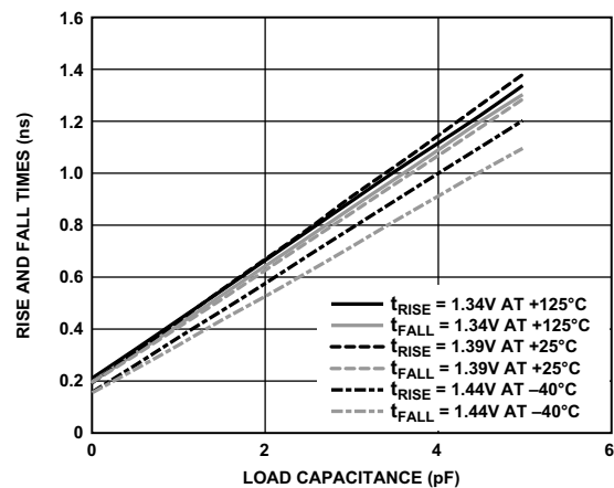
Figure 82. Driver Type B and Driver Type C Rise and Fall Times (10% to 90%) vs. Load Capacitance for DDR3L at 100 \Omega
