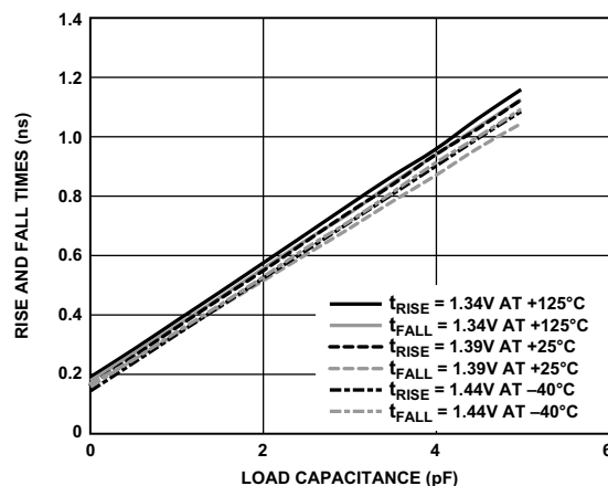
Figure 81. Driver Type B and Driver Type C Rise and Fall Times (10% to 90%) vs. Load Capacitance for DDR3L at 90 \Omega
