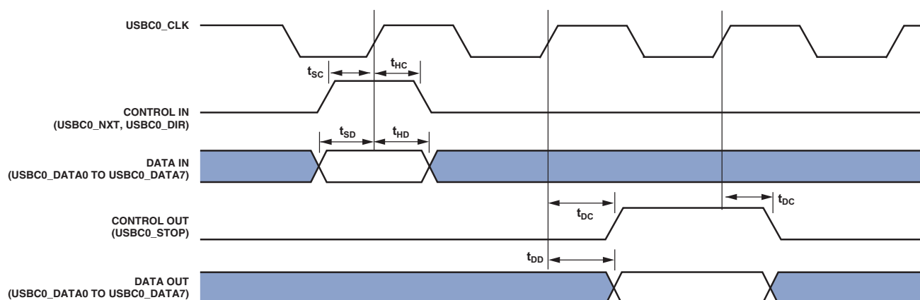
Figure 34. USB Timing
