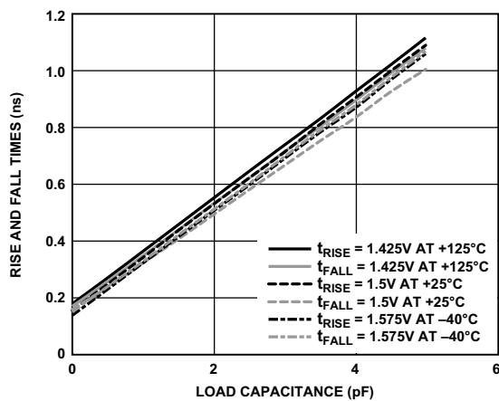
Figure 79. Driver Type B and Driver Type C Typical Rise and Fall Times (10% to 90%) vs. Load Capacitance for DDR3 at 90 \Omega
