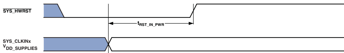
Figure 8. Power-Up Reset Timing
