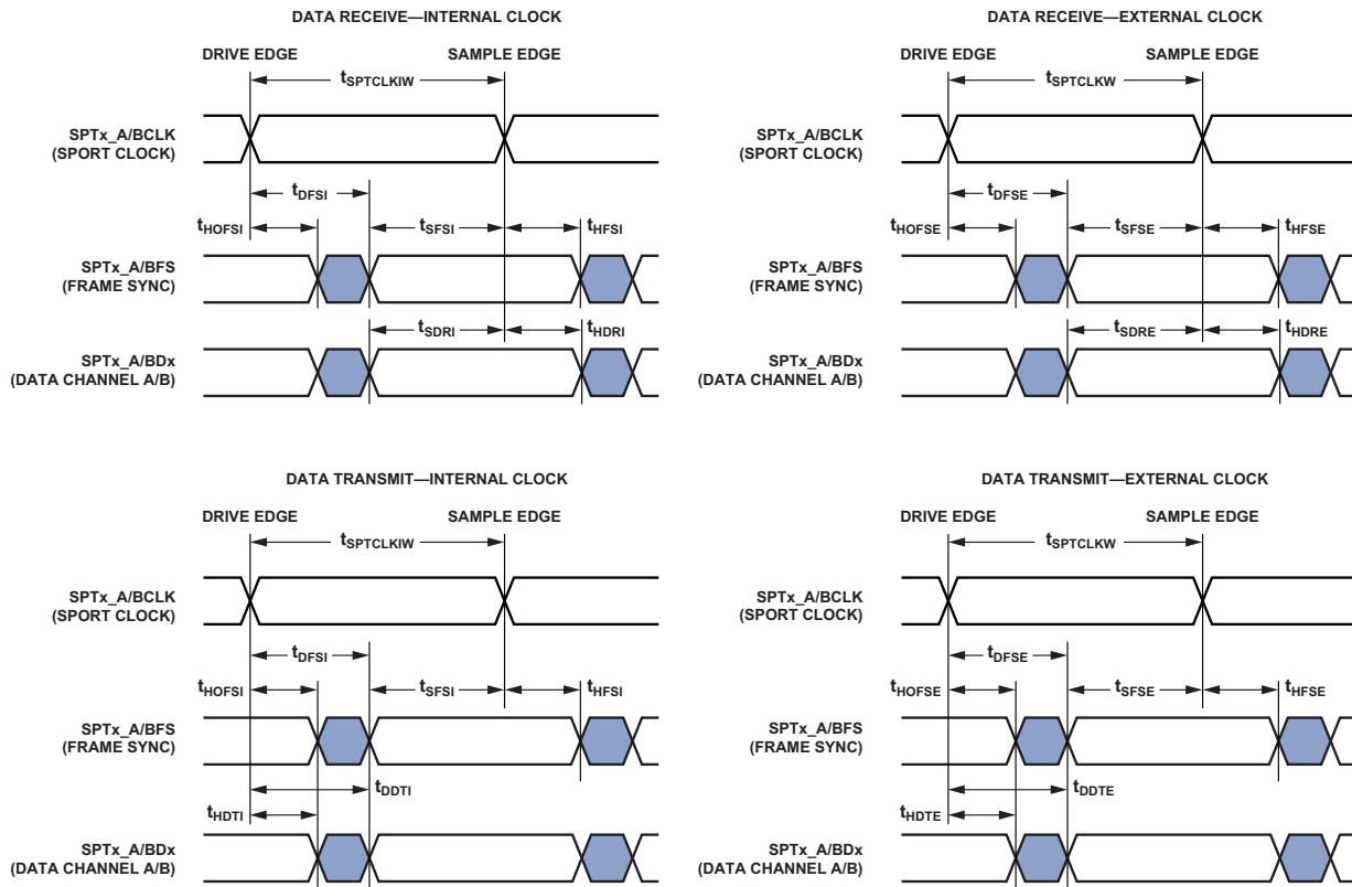
Figure 15. SPORTs
