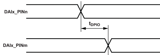
Figure 32. DAI Pin to DAI Pin Direct Routing
