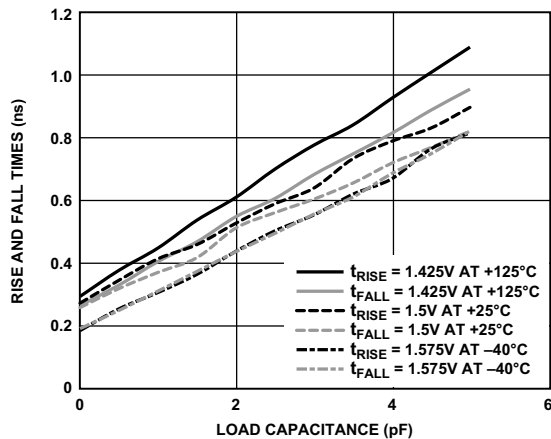
Figure 80. Driver Type B and Driver Type C Typical Rise and Fall Times (10% to 90%) vs. Load Capacitance for DDR3 at 100 \Omega
