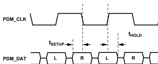
Figure 62. PDM Timing
