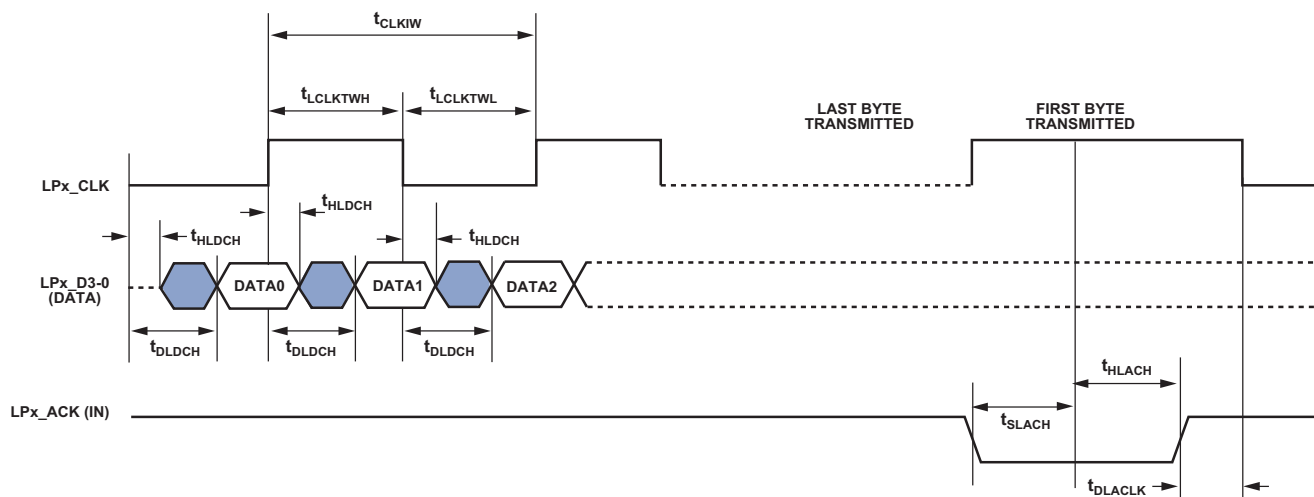
Figure 14. LPs DDR—Transmit
