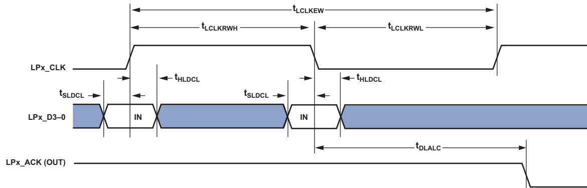
Figure 13. LPs DDR—Receive
