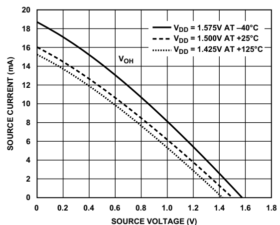
Figure 68. Driver Type B and Driver Type C (DDR3 Drive Strength 100 \Omega )
