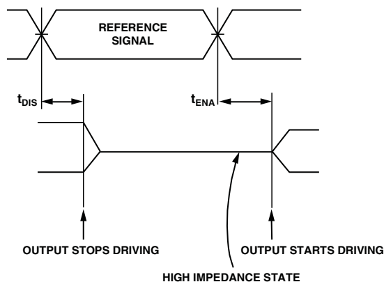
Figure 75. Output Enable/Disable
