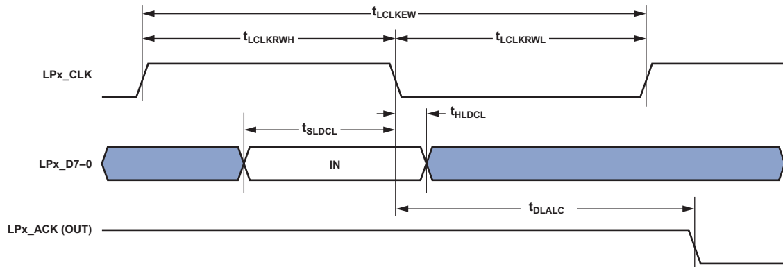
Figure 13. LPs—Receive
