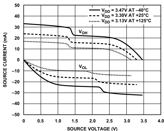
Figure 42. Driver Type A Current for All Pins Operating at Less Than or Equal to 62.5 MHz (3.3 V V_{DD\_EXT} )
