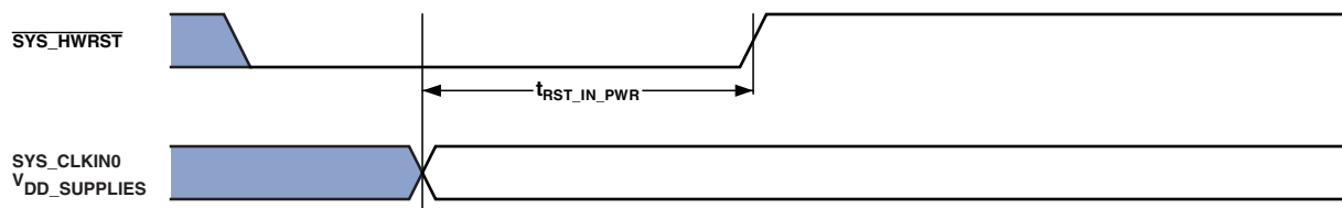
Figure 10. Power-Up Reset Timing
