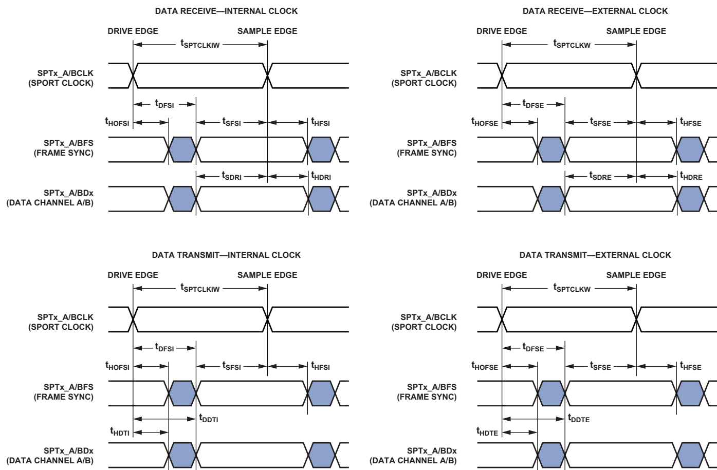
Figure 15. SPORTs
