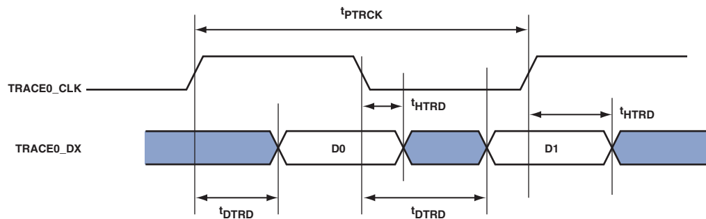
Figure 40. Trace Timing
