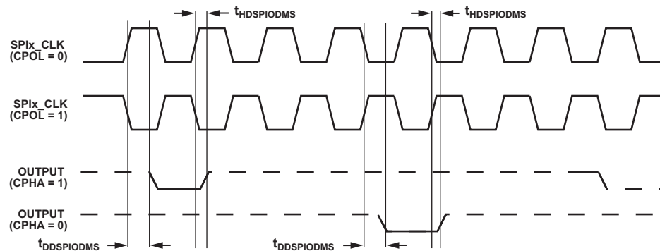
Figure 25. ODM Slave Mode
