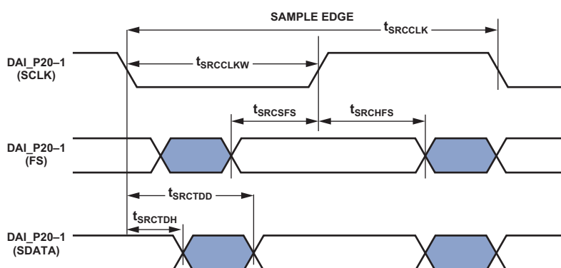
Figure 27. ASRC Serial Output Port Timing
