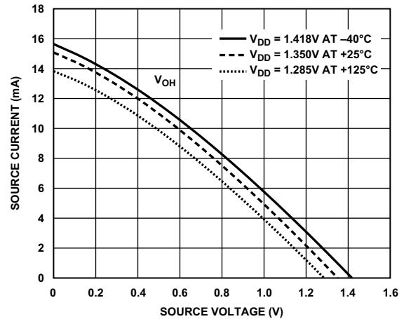
Figure 43. Driver Type B and Driver Type C (DDR3L Drive Strength 100 Ω)
