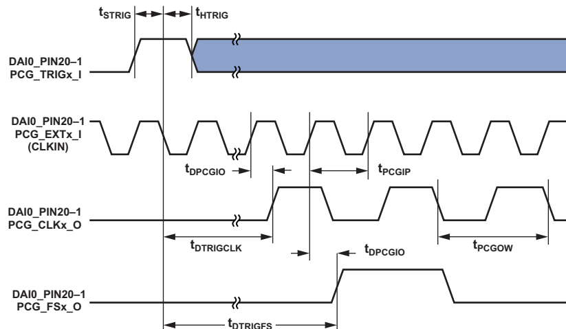
Figure 26. PCG (Direct Pin Routing)
