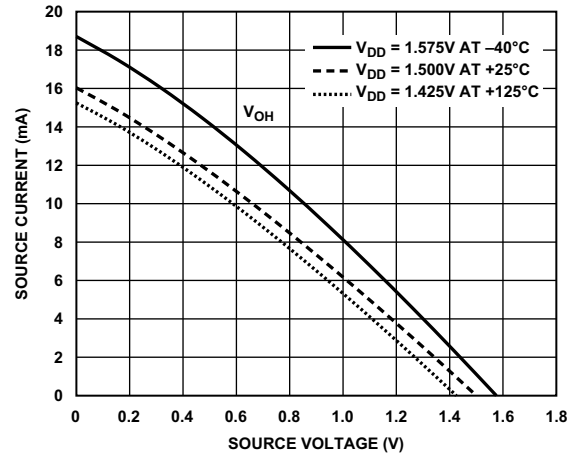
Figure 41. Driver Type B and Driver Type C (DDR3 Drive Strength 100 Ω)
