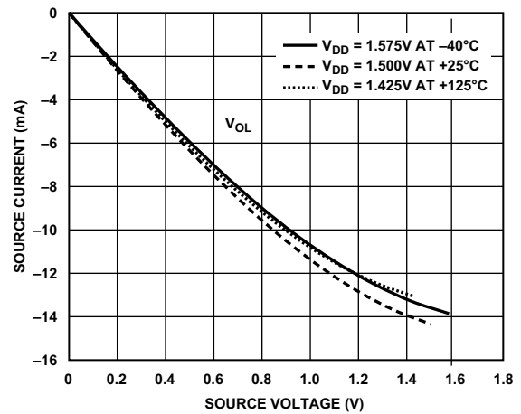
Figure 42. Driver Type B and Driver Type C (DDR3 Drive Strength 100 Ω)
